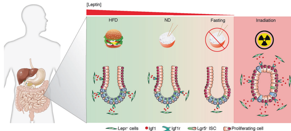
Fig. 9 The working model of the mechanism by which Lepr + cells modulate ISC under conditions of HFD regime, fasting regime and post-irradiation. Lepr + cells are identified as a mesenchymal niche source for ISCs, and they can sense diet alterations to modulate ISCs via a stromal IGF1–epithelial IGF1R axis. Upon fasting, the abundance of Lepr + cells dramatically decreases due to the reduced Leptin, leading to the reduction of Lepr + cell-secreted Igf1. Consequently, the proliferation of ISCs and progenitor cells declines under fasting regime. Conversely, the abundance of Lepr + cells increases upon HFD regime and post-irradiation, and the increased Lepr + cells promote the proliferation of ISCs and progenitor cells by enhancing the secretion of Igf1.
