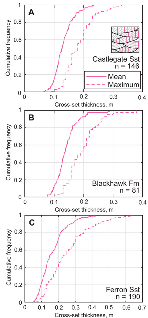
Fig. 4. The cumulative frequency of the mean, median and maximum cross-set thickness for (A) the Castlegate Sandstone, (B) the Blackhawk Formation, and (C) the Ferron Sandstone. The solid pink line indicates the measured mean and the dashed pink line indicates the measured maximum. n indicates the number of cross-sets in which thickness distributions were measured, and therefore the number of cross-sets from which a mean and maximum thickness were subsequently extracted. The inset in A is a schematic representation of how thickness distributions were measured within each cross-set.
