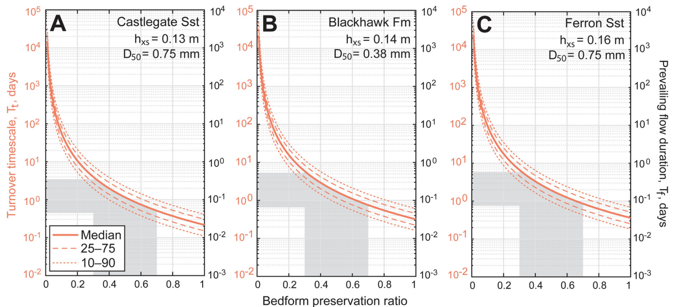
Fig. 8. Turnover timescales, T_t , reconstructed for the Castlegate Sandstone, Blackhawk Formation and Ferron Sandstone using a range of preservation ratios. For these purposes, the mean cross-set thickness ( h_{xs} ) and median grain-size ( D_{50} ) for each geologic formation have been used (i.e., the mean and median across all measured cross-set distributions). The solid orange line indicates the median T_t reconstructed for each bedform preservation ratio, the dashed orange lines indicate the 25 th –75 th percentile range of T_t values reconstructed for each bedform preservation ratio, and the dotted orange lines indicate the 10 th –90 th percentile range of T_t values reconstructed for each bedform preservation ratio, which we offer as plausible spreads of values for mean T_t (see Supplementary Methods). The grey region highlights the range of median T_t values associated with a plausible range of bedform preservation ratios; steady-state bedform preservation ratios are \sim 0.3 , and Leary and Ganti (2020) documented that higher bedform preservation ratios may extend up to \sim 0.7 during flash floods. On the right y axis, we show reconstructed prevailing flow durations, T_f , for the scenario in which T_f is a factor of 10 smaller than the reconstructed bedform turnover timescale.
