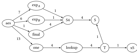
Figure 5: Module dependency graph of the AES-256 benchmark.
