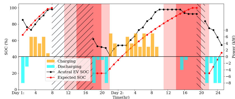
Figure 11. EV simulation of proposed HEMS.
