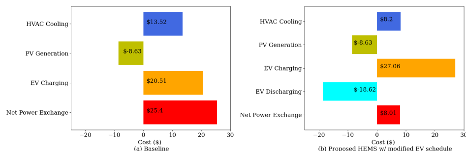
Figure 13. Total energy cost breakdown between the baseline and the proposed HEMS with modified EV schedule.
