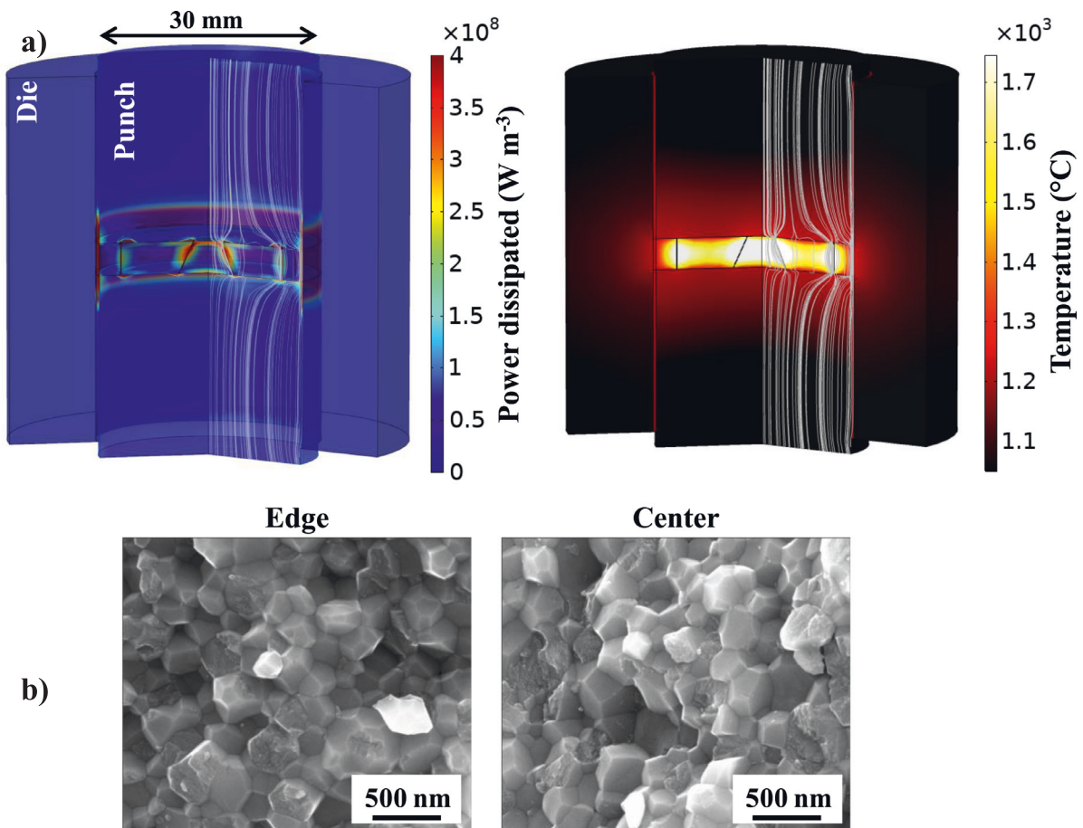
Fig. 4. Physical field uniformity and correlation with obtained microstructures. The upper part (a) shows the temperature distribution and electric current lines during the electric current peak, the lower part (b) represents the SEM fracture images in the center and at the edge of the sintered sample which demonstrate a homogeneous microstructure with grain size clearly lower than 500 nm.
