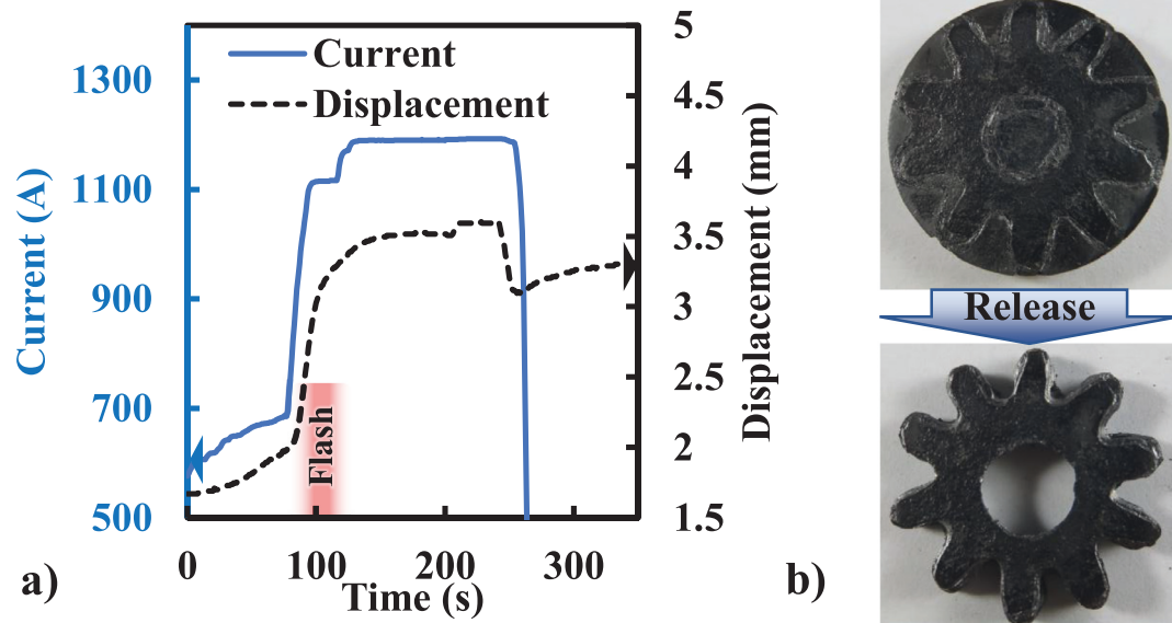
Fig. 3. Flash sintering of 30 mm zirconia gear. a) Current and displacement curves recorded during the flash spark plasma sintering experiment b) the upper part shows the sintered pellet where the gear shape appears along with the sacrificial parts and graphite foils interface, the lower part shows the released gear shape after ejection of the sacrificial parts.
