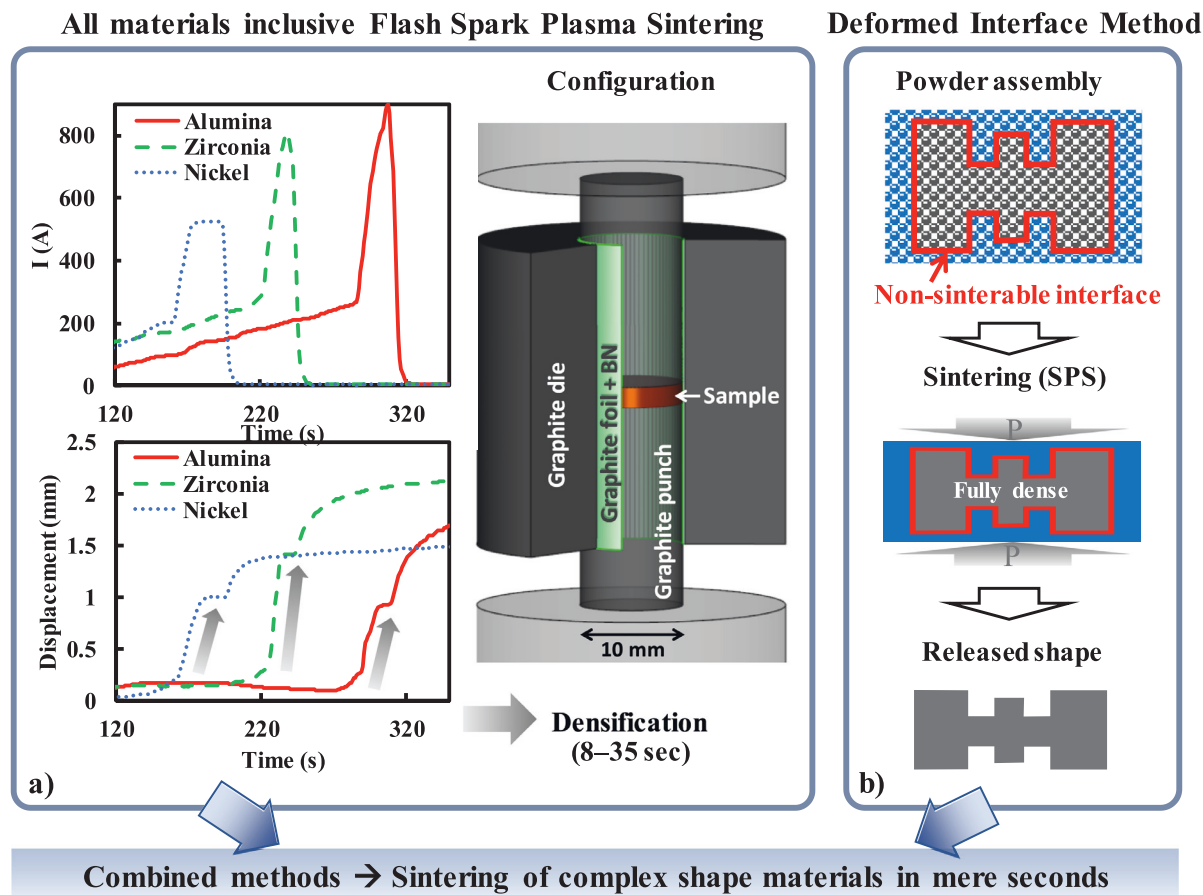
Fig. 1. Concept of complex shape flash sintering. The ultra-rapid complex shape sintering method integrates two coupled approaches: a) the flash spark plasma sintering conditions and configuration [8] b) the complex shape deformed interface approach [18].
