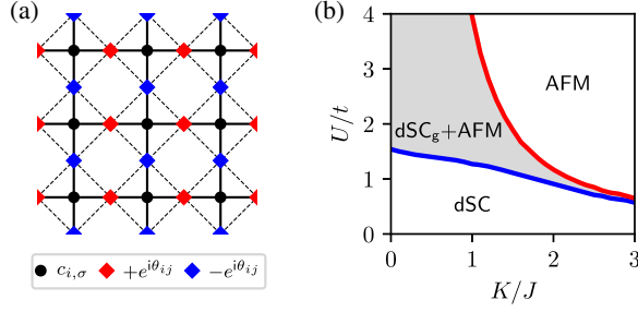
FIG. 1. The lattice model and mean-field phase diagram at V/t = 0.5 . (a) The lattice model. Fermions (black circle dots) live on a square lattice with nearest hopping and on-site Hubbard interaction U . Rotors (colored square dots) live on the bonds of the same square lattice described by a quantum rotor Hamiltonian. Rotors coupled to fermion pairing operators with the d -wave form indicated by different signs ( \tau_{ij} = \pm 1 ) in front of e^{i\theta_{ij}} . (b) Mean-field phase diagram. dSC stands for the nodal d_{x^2-y^2} superconductor, AFM for the antiferromagnetic insulator, and dSC_g + AFM for the coexisting gapped d -wave superconductor and antiferromagnetic insulator.
