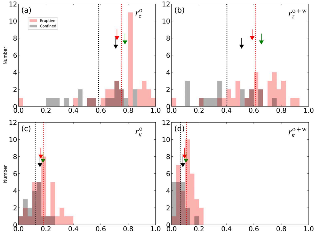
Figure 2. Histograms of (a) r_{\tau}^o , (b) r_{\tau}^{o+w} , (c) r_{\kappa}^o , and (d) r_{\kappa}^{o+w} for eruptive events (shaded red) and confined events (shaded gray). Red (black) vertical dashed lines indicate the mean value of the variables for eruptive (confined) events. The arrows colored red, green, and black indicate the value that events #35, #36, and #37 host, respectively.
