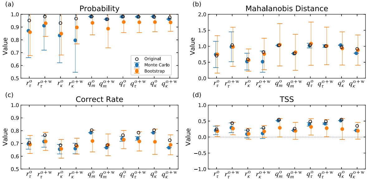
Figure 3. The comparison of the resulting DA metrics for the r -scheme ( r_\tau^o , r_\tau^{o+w} , r_\kappa^o , and r_\kappa^{o+w} ) and q -scheme ( q_m^o , q_m^{o+w} , q_\tau^o , q_\tau^{o+w} , q_\kappa^o , and q_\kappa^{o+w} ). The metrics are (a) the probability that the two groups are sampled from two distinct populations, (b) Mahalanobis distance, (c) correct rate, and (d) TSS. The unfilled black circles indicate the value yielded through the n - 1 cross-validation. The data points and the associated error bars colored in blue (orange) stand for the estimations yielded by the Monte Carlo algorithm (bootstrap method). A horizontal dashed line in (d) divides the space of positive and negative skills for the classification.
