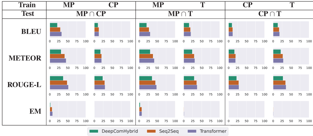
Figure 9: Results of comment generation models with filtering near-duplicates using the same_summary configuration, on TestC sets.
