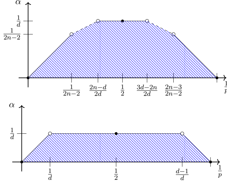
FIGURE 2. Conjectured range of A_\gamma: L^p(\mathbb{R}^n) \rightarrow L_\alpha^p(\mathbb{R}^n) boundedness for \gamma of maximal type d . The upper diagram corresponds to d < 2n - 2 whilst the lower diagram corresponds to d \geq 2n - 2 .
