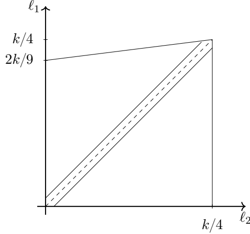
FIGURE 4. Setting \ell = \ell_1 for a_{k,\ell,1} and \ell = \ell_2 for a_{k,\ell,\iota} , 2 \leq \iota \leq 4 , one can interpret the decomposition (6.10) in the (\ell_2, \ell_1) -plane as follows. The symbols a_{k,\ell,1} correspond to horizontal lines in the lower triangle, whilst the symbols a_{k,\ell,2} correspond to vertical lines in the diagonal and upper triangle whenever u_2(\xi) > 0 . If u_2(\xi) < 0 , the symbols a_{k,\ell,3} correspond to vertical lines in the fattened diagonal, the symbols a_{k,\ell,4} correspond to vertical lines in the upper triangle (under the additional condition that |s - \theta_1(\xi)| \gtrsim 2^{-\ell_2} ) and the symbols b_{k,\ell} correspond to integer points in the upper triangle (under the additional condition that |s - \theta_1(\xi)| \lesssim 2^{-\ell_2} ).
