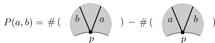
FIGURE 24. A count that determines how a and b q -commute through the application of height exchange moves.
