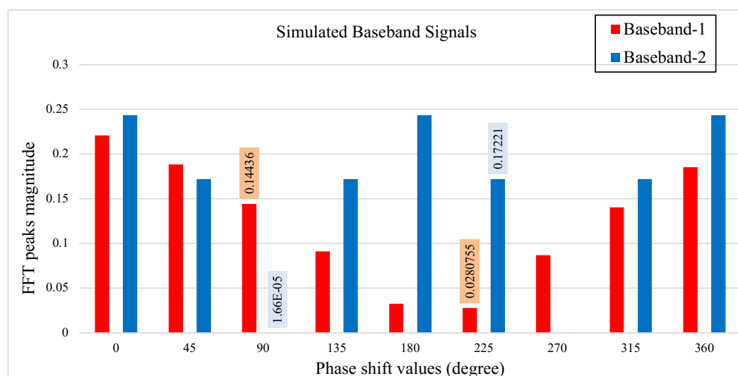
Figure 1. The figure shows two simulated receiving signals, 0.2 Hz baseband-1 and 0.3 Hz baseband-2, with phase sweeping between \theta_{ps} = 0^\circ to \theta_{ps} = 360^\circ , incremented at \Delta\theta_{ps} = 45^\circ per step.
