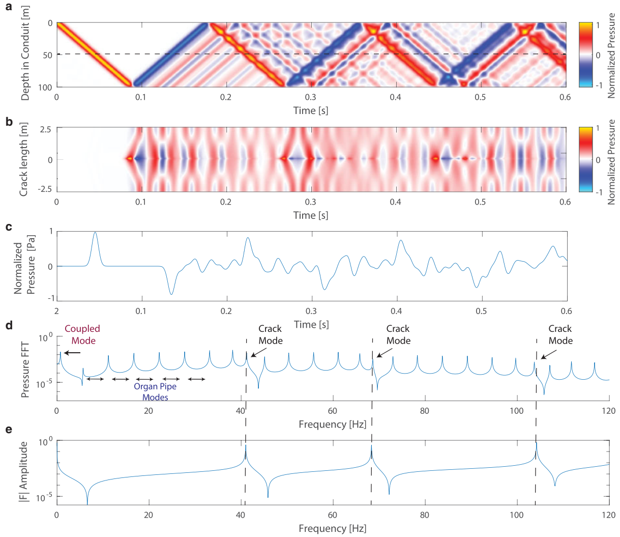
Fig. 4. Spatial time series and frequency spectra for resulting wave motion in an englacial geometry with a conduit connected to a basal crack (assuming fully developed flow). (A) Similar to Fig. 3 but showing pressure time series throughout the conduit–crack network. (B) Spatial time series in the crack. (C) Pressure time series in the conduit taken at 50 m depth noted as the dashed line in panel (A). (D) Frequency spectrum of the time series shown in (C). In this frequency spectra, we note the coupled frequency at 0.75 Hz, crack wave modes at frequencies 41, 68 and 103 Hz, and many harmonics of the fundamental organ pipe frequency at 5.6 Hz. (E) Normalized crack impedance |F| for the basal crack, where |F| maxima correspond to observed crack wave frequencies in the conduit.
