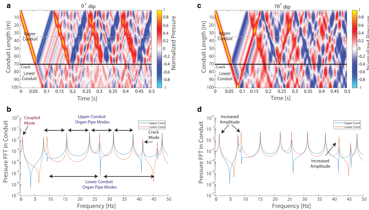
Fig. 7. Spatial time series and frequency spectra for two middle crack models with the same geometric parameters and forcing as the coupled basal crack simulation in Fig. 4, except that the crack is located at 70 m down the conduit and varies in dip between the two simulations. (A) Spatial time series for a crack dipping at 0^\circ . (C) Spatial time series for a crack dipping at 70^\circ . (B) Frequency spectra for a crack dipping at 0^\circ . (D) Frequency spectra for a crack dipping at 70^\circ . The thick black line in (A) and (C) represents the location of the crack and the gray dashed lines represent the location of the time series in the upper and lower conduits that are Fourier transformed to create the spectra in (B) and (D).
