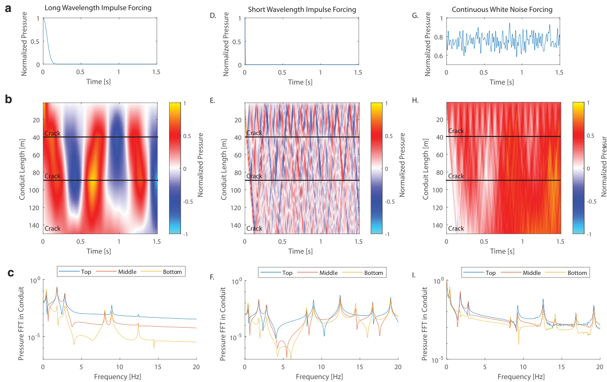
Fig. 9. Excitation of resonant modes from different source-time functions in a three crack system where the cracks are at depths of 40, 90 and 150 m. All other model parameters are the same as previous experiments and assuming fully developed flow. Left column: A long wavelength Gaussian excitation, with a scaled wavelength of 130 m. (A) Forcing function for the long wavelength model run. (B) Spatial time series for the long wavelength model run. (C) Frequency spectra for the long wavelength model run showing the FFT of time series taken at 20, 65 and 120 m. Middle column: A short wavelength excitation, with a scaled wavelength of 10 m. (D) Forcing function for the short wavelength model run. (E) Spatial time series for the short wavelength model run. (F) Frequency spectra for the short wavelength model run showing the FFT of time series taken at 20, 65 and 120 m. Right column: A simulated white noise continuous excitation, comprised of 2000 sine waves with random initial phase and a small amount of numerical noise. (G) Forcing function for the continuous forcing model run. (H) Spatial time series for the continuous forcing model run. (I) Frequency spectra for the continuous forcing model run showing the FFT of time series taken at 20, 65 and 120 m.
