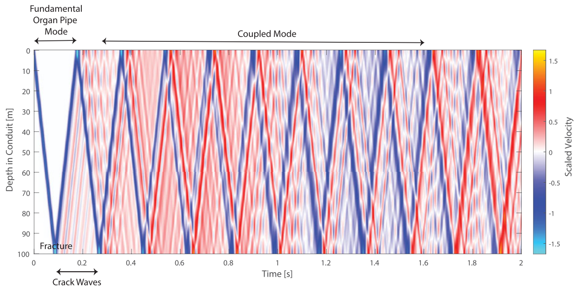
Fig. 3. Fluid particle velocity ( u_z ) throughout the conduit in time, for a basal crack system with conduit length L = 100 m, radius R = 10 cm, a symmetric crack of length L_x = 5 m and opening of w_0 = 1 cm. The center of the Gaussian excitation pulse is at 0 s model time with a scaled wavelength of 10 m. Following excitation we follow the propagating tube wave down the conduit until it reaches the basal crack at 100 m. When the tube wave reaches the crack, most of the energy is reflected and subsequently resonates at the fundamental organ pipe frequency. Energy that enters the crack is transmitted back into the conduit in the form of crack waves (first seen from \sim 0.1 – 0.3 s). Although wave motion becomes more complex through time, we note a full conduit velocity polarity change at \sim 1 – 1.2 s. This bulk motion in the fluid shows the long period coupled mode in the basal crack system.
