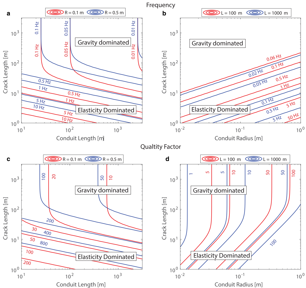
Fig. 6. Coupled mode frequency and quality factor for the range of glacial parameters in Table 1. (A and B) Frequency contours for R = 0.1 and 0.5 m, and L = 100 and 1000 m. (C and D) Quality factor contours for R = 0.1 and 0.5 m, and L = 100 and 1000 m. In all panels, transitions to the gravity-dominated limit can be seen where the frequency and quality factor lose crack length dependence. Panel (B) in particular shows no frequency variation for crack lengths above the 0.06 Hz (red) and 0.02 Hz (blue) contour. Conduit lengths and radii were chosen as proxies for an alpine and ice-sheet environment.
