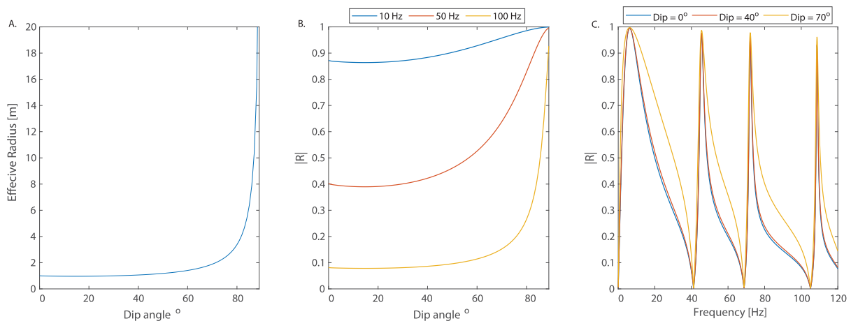
Fig. 8. Effects of crack dip angle. (A) Role of crack dip on effective radius of a tabular crack intersecting a central conduit. (B and C) Variation of reflection coefficient (Eqn (43)) with dip angle and frequency, geometric parameters similar to Fig. 7.
