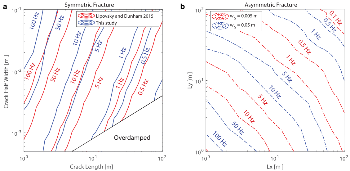
Fig. 2. Fundamental crack resonant frequencies for symmetric and asymmetric cracks. (A) Fundamental mode of a symmetric tabular crack, comparing the 2-D model (one length dimension and opening) of Lipovsky and Dunham (2015) (red contours) to the 3-D model studied here (blue contours). The over-damped region is determined from Lipovsky and Dunham (2015); no resonance occurs in this part of parameter space. (B) Variation of the fundamental mode for an asymmetric 3-D crack for two different crack length dimensions L_x and L_y . Where red contours represent a crack thickness of 0.005 m and blue contours represent results for a crack thickness of 0.05 m. Undulations in the contours reflect finite numerical resolution of crack storativity, leading to \sim 5\% uncertainty in crack dimensions.
