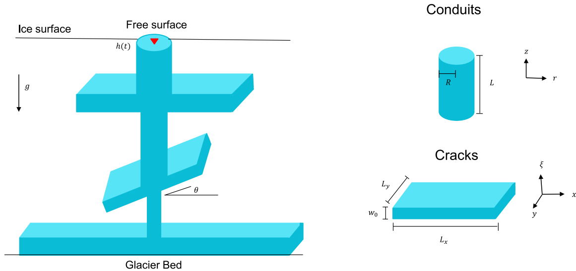
Fig. 1. Idealized model of the englacial system showing multiple cracks branching from a central conduit. Cracks are defined by two length scales L_x and L_y and opening w_0 . Conduit sections are defined by a length L and a radius R . Cracks may also be dipping at an angle \theta with respect to the conduit axis. The free surface is denoted by a red triangle. h(t) is the height of the water surface in reference to an unperturbed fluid surface at atmospheric pressure.
