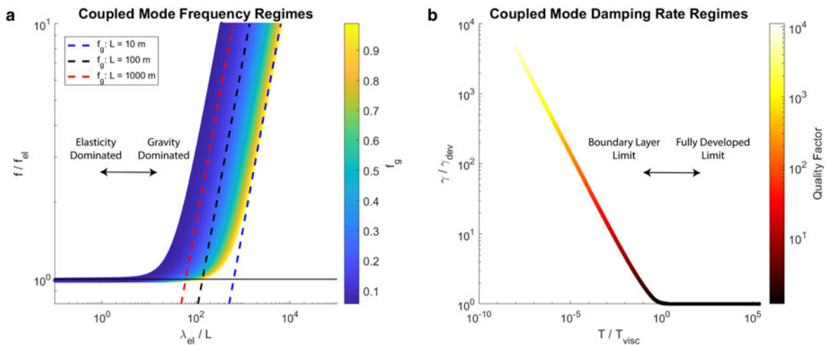
Fig. 5. Coupled mode frequency and damping rate regimes. (A) Dominant restoring force as a function of frequency f for the coupled mode in a basal crack system. In the elastic limit, the coupled mode frequency is f_{el} = (1/2\pi)\sqrt{(A_c/\rho_0 C_1)/L} , while in the gravity limit frequency follows f_g = (1/2\pi)\sqrt{g/L} . The x-axis shows the wavelength \lambda_{el} = c_T/f_{el} normalized by conduit length L . The dashed lines represent the gravity limit frequency for three different conduit lengths of 10, 100 and 1000 m. This highlights where the data collapse onto the gravity limit. (B) Quality factor of the coupled mode is controlled by the ratio of mode period and momentum diffusion time across the conduit T_{visc} = R^2 \rho_0 / \mu . The y-axis shows cross-sectionally averaged shear stress in the conduit (Eqn (39)) normalized by the fully developed limit \gamma_{dev} = 4\mu/\rho_0 R^2 = 4/T_{visc} . This illustrates the importance of a boundary layer treatment of viscous damping for assessing quality factors in the glacial environment.
