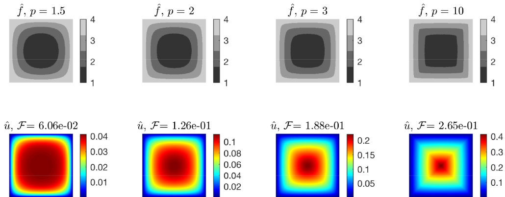
FIGURE 13. The minimizer \hat{f} and its corresponding \hat{u} on a square for p = 1.5, 2, 3, 10 .
