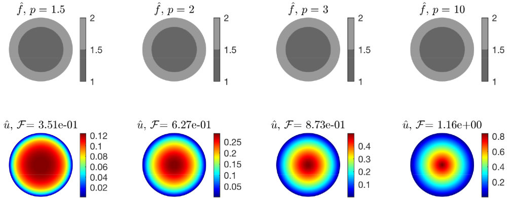
FIGURE 3. The minimizer \hat{f} and its corresponding \hat{u} on a disk for p = 1.5, 2, 3, 10 .
