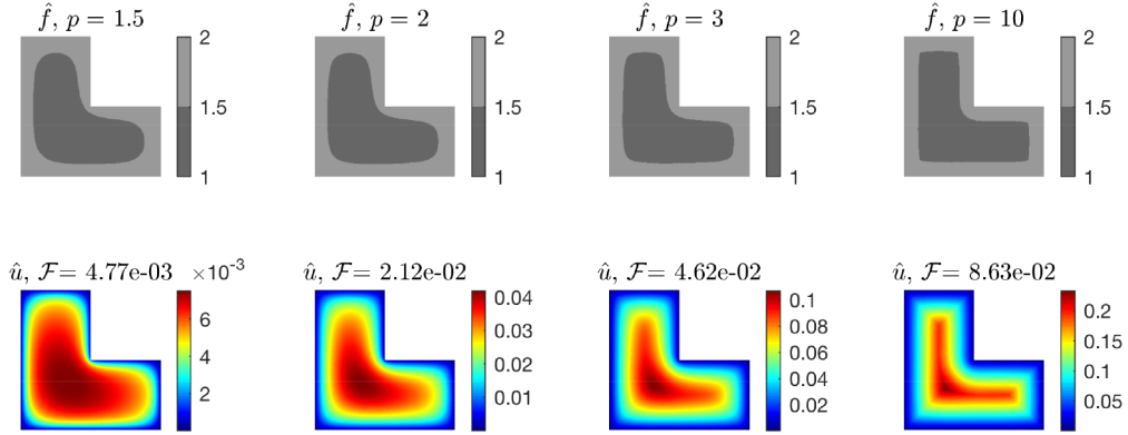
FIGURE 5. The minimizer \hat{f} and its corresponding \hat{u} on a L-shaped domain for p = 1.5, 2, 3, 10 .
