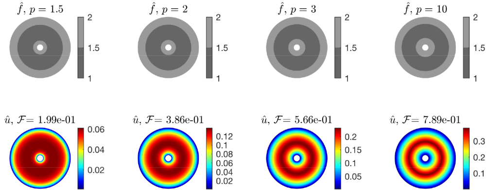
FIGURE 7. The minimizer \hat{f} and its corresponding \hat{u} on an annulus for p = 1.5, 2, 3, 10 .
