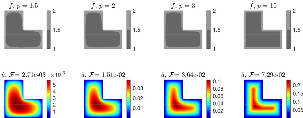
FIGURE 10. The minimizer \hat{f} and its corresponding \hat{u} on a L-shaped domain for p = 1.5, 2, 3, 10 .
