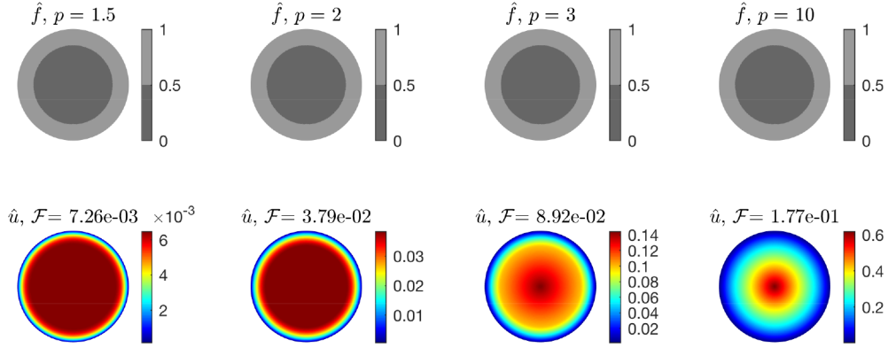
FIGURE 8. The minimizer \hat{f} and its corresponding \hat{u} on a disk for p = 1.5, 2, 3, 10 .
