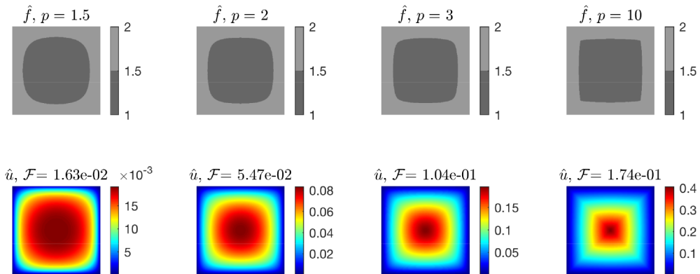
FIGURE 4. The minimizer \hat{f} and its corresponding \hat{u} on a square for p = 1.5, 2, 3, 10 .
