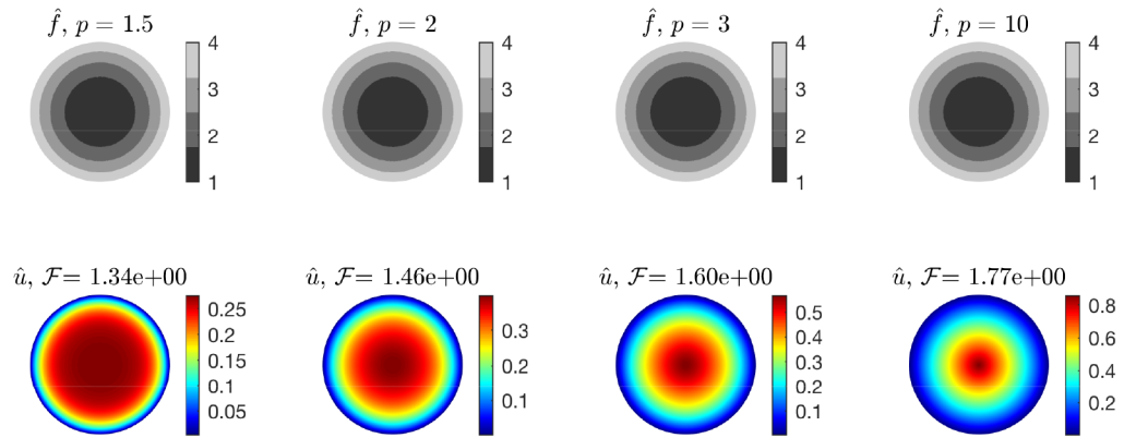
FIGURE 12. The minimizer \hat{f} and its corresponding \hat{u} on a disk for p = 1.5, 2, 3, 10 .
