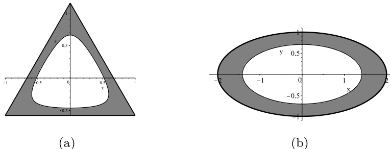
FIGURE 1. Nearly optimal solutions in the low contrast regime with p = 2 . The set E_\tau with |E_\tau| = |\Omega|/2 is shown in gray.
