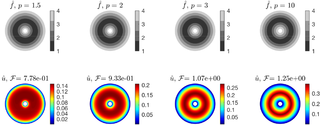
FIGURE 14. The minimizer \hat{f} and its corresponding \hat{u} on an annulus for p = 1.5, 2, 3, 10 .
