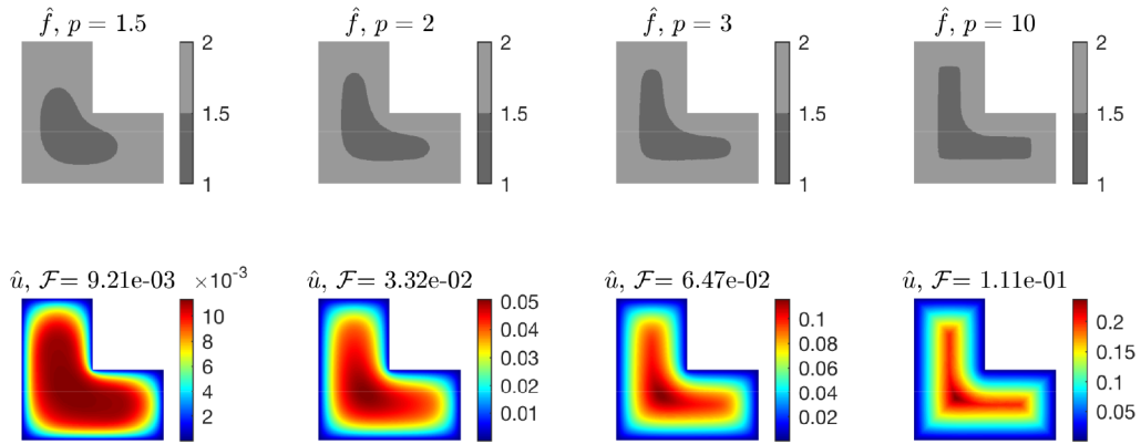
FIGURE 11. The minimizer \hat{f} and its corresponding \hat{u} on a L-shaped domain for p = 1.5, 2, 3, 10 .
