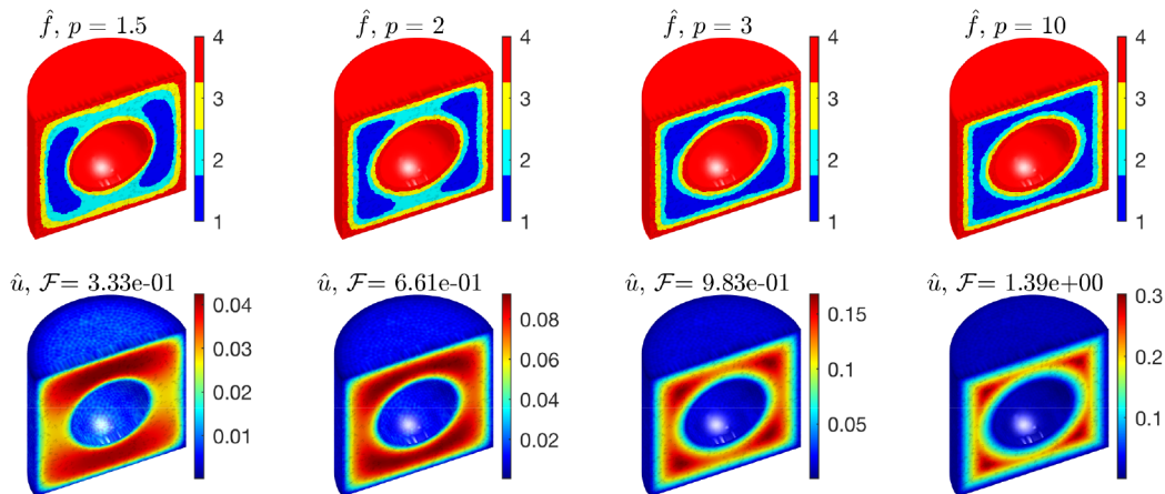
FIGURE 16. The minimizer \hat{f} and its corresponding \hat{u} on a cylinder with a hole for p = 1.5, 2, 3, 10 .
