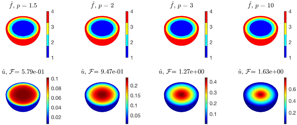
FIGURE 15. The minimizer \hat{f} and its corresponding \hat{u} on the unit sphere for p = 1.5, 2, 3, 10 .
