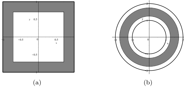
FIGURE 2. Nearly optimal solutions when p \rightarrow \infty . The set F_\tau with |F_\tau| = |\Omega|/2 is shown in gray.
