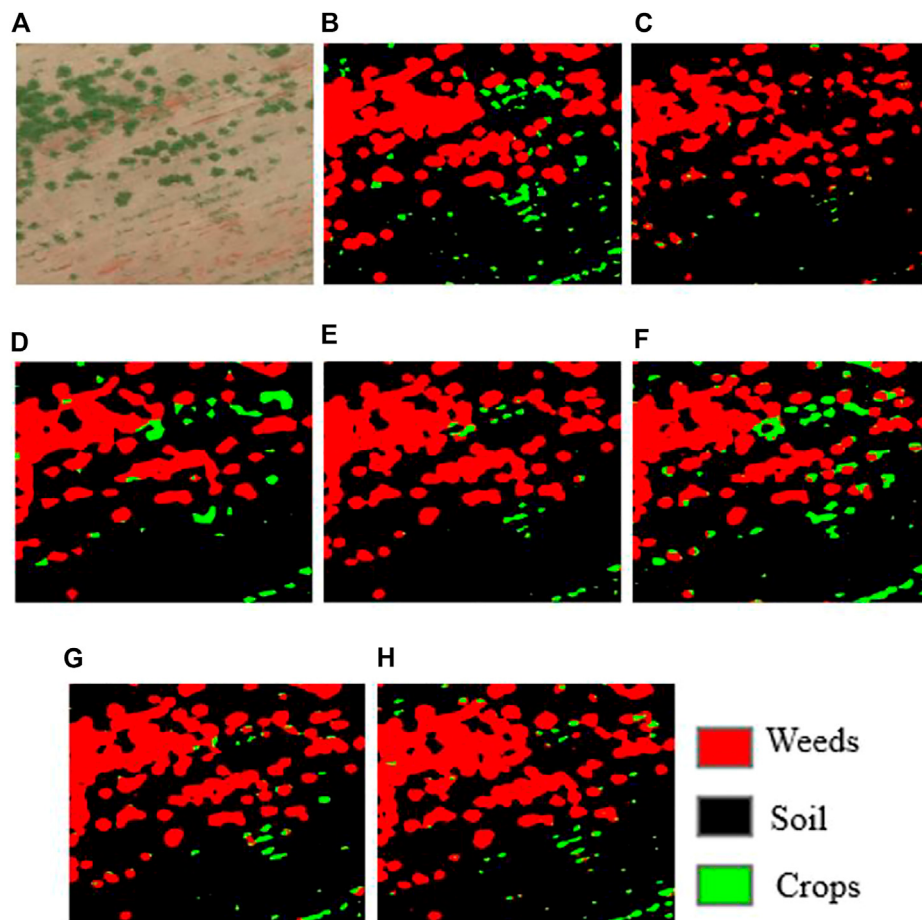
FIGURE 8 | Sample qualitative results were achieved for sugarcane dataset. (A) input images; (B) groundtruth, (C) SegNet, (D) FCN-32s, (E) FCN-16s, (F) FCN-8s, (G) U-Net, (H) Deeplabv3++ result.
