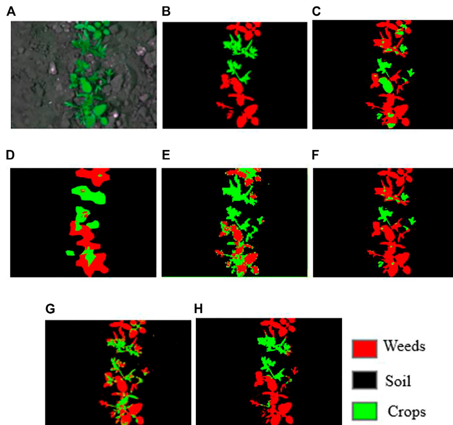
FIGURE 7 | Sample qualitative results were achieved for CWFD. (A) input images; (B) groundtruth, (C) SegNet, (D) FCN-32s, (E) FCN-16s, (F) FCN-8s, (G) U-Net, (H) DeepLabV3++.
