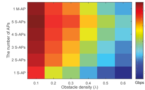
Fig. 5. Throughput performance with a single M-AP and multiple S-APs.
