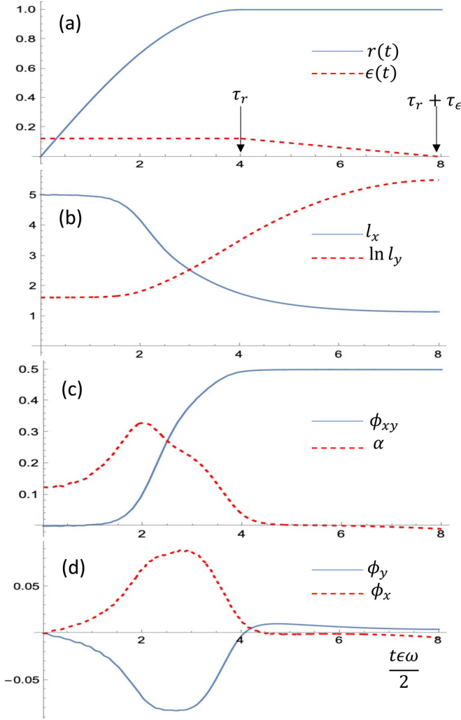
FIG. 5. Model and wave-function Ansatz parameters as a function of time in the protocol where \varepsilon is ramped to zero. All parameters are dimensionless. (a) r(t) (blue, solid) and \varepsilon (red, dashed). (b) l_x(t) (blue, solid) and \ln(l_y(t)) (red, dashed); ramping \varepsilon \rightarrow 0 cuts off the exponential growth of l_y that was seen in Fig. 2. (c) \phi_{xy}(t) (blue, solid) again saturates at 0.5 and \alpha(t) (red, dashed) saturates at a negative value, which depends on the ramp. (d) \phi_y(t) (blue, solid) and \phi_x(t) (red, dashed) saturate at \pm\alpha/2 . All parameters are subsequently time independent.
