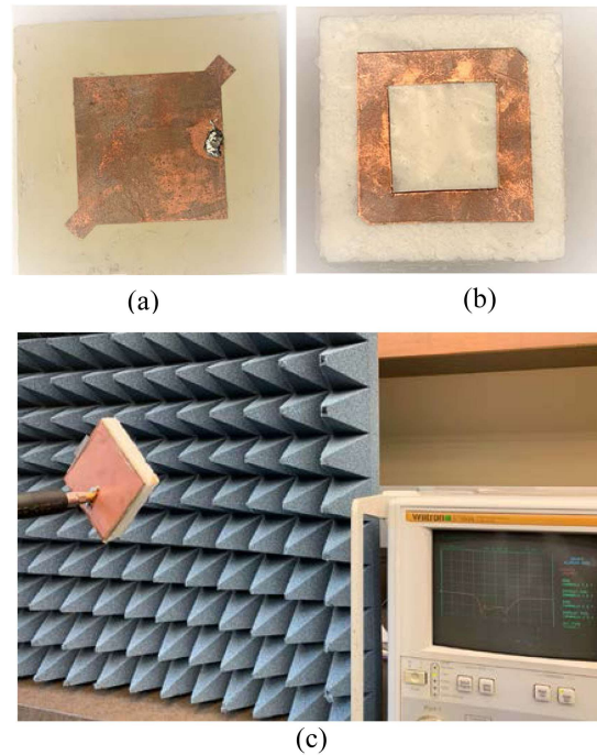
Figure 13. (a) Driven patch of the fabricated antenna. (b) Top view of the fabricated antenna. (c) Fabricated antenna under test.
