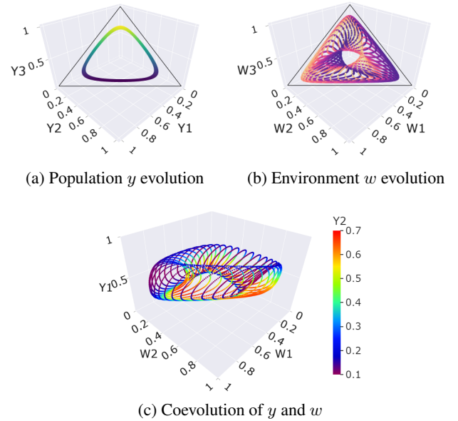
Figure 1: Poincaré recurrence in a time-evolving generalized Rock-Paper-Scissors model.
