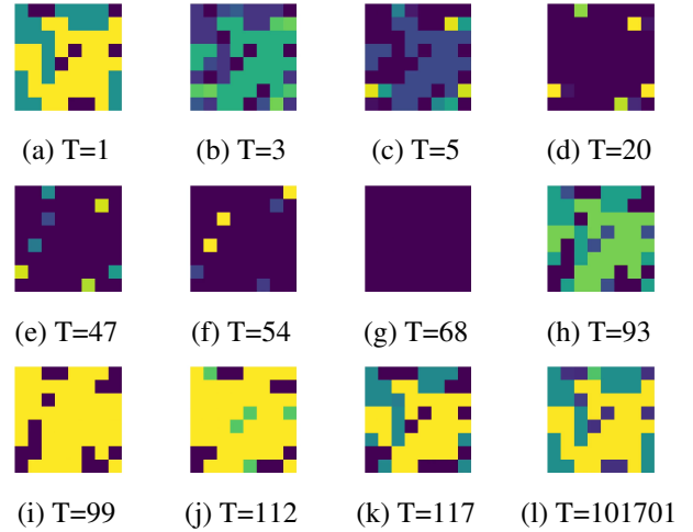
Figure 4: Sequence of Pikachu images showing approximate recurrence in an 8 \times 8 zero-sum polymatrix game, where the changing color of each pixel on the grid represents the strategy of the player over time.
