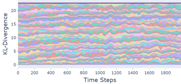
Figure 3: Weighted KL divergence for 25 cluster (100 player) time-evolving zero-sum game.
