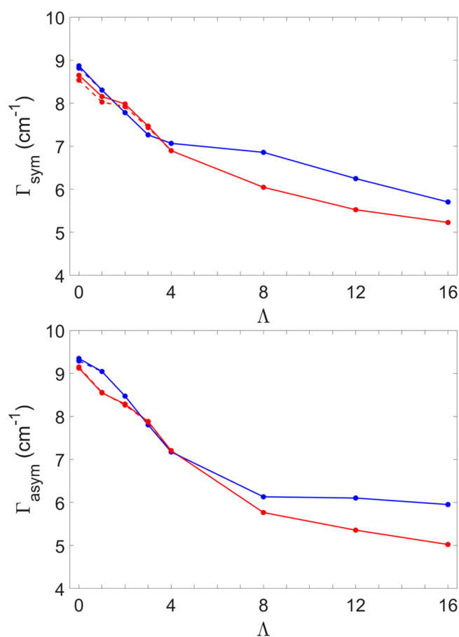
Figure 5. Average values of resonance widths in symmetric (top frame) and asymmetric (bottom frame) ozone molecules for J = 28 . The meaning of lines and colors is the same as in Figure 4.
