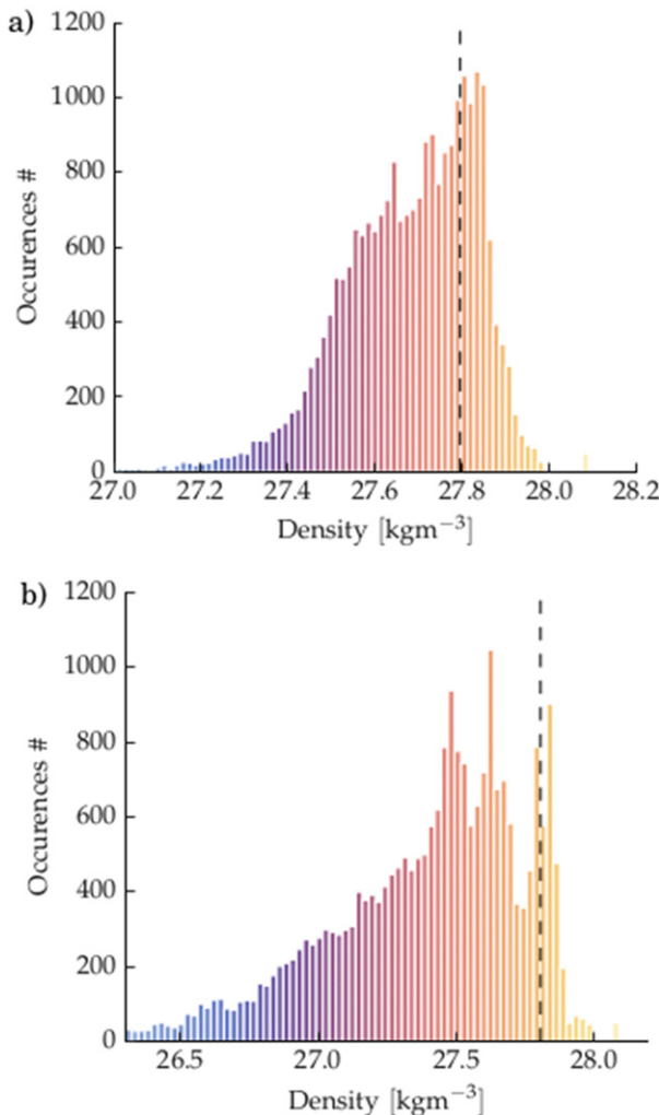
FIG. 10. Histogram of vortex core densities, extracted at depth of the maximum vorticity in the vortex center of all anticyclones identified in the central Lofoten Basin (within the 3000-m depth contour) during (a) winter and (b) summer. The dashed black lines show the time-mean density of the LV core at 400-m depth during the respective seasons.
