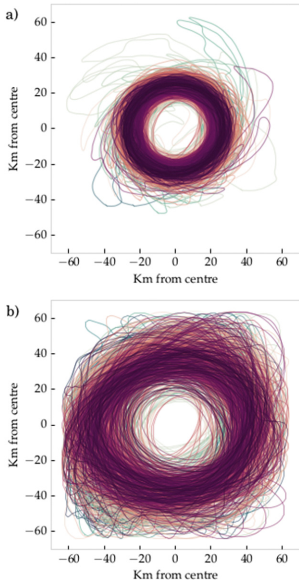
FIG. 3. (a) OW = 0 contours and (b) outermost SSH contour extracted daily around the LV center found each day during 1995–99, the first 4 years after the spinup period. Colors are arbitrary.
