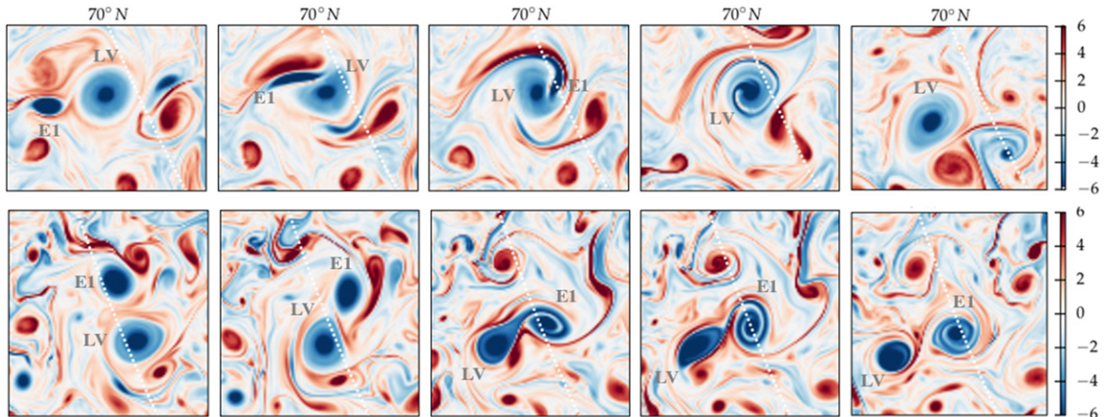
FIG. 12. Sequences of horizontal maps of relative vorticity at a 400-m depth displaying examples of (top) an asymmetric merger where the approaching vortex is smaller in size, but stronger than the LV, and (bottom) a partial merger event, where the LV is repelled from the approaching vortex (E1) after a brief interaction. The LV and the approaching vortex (E1) are labeled in all columns. The white dashed line shows 70°N.
