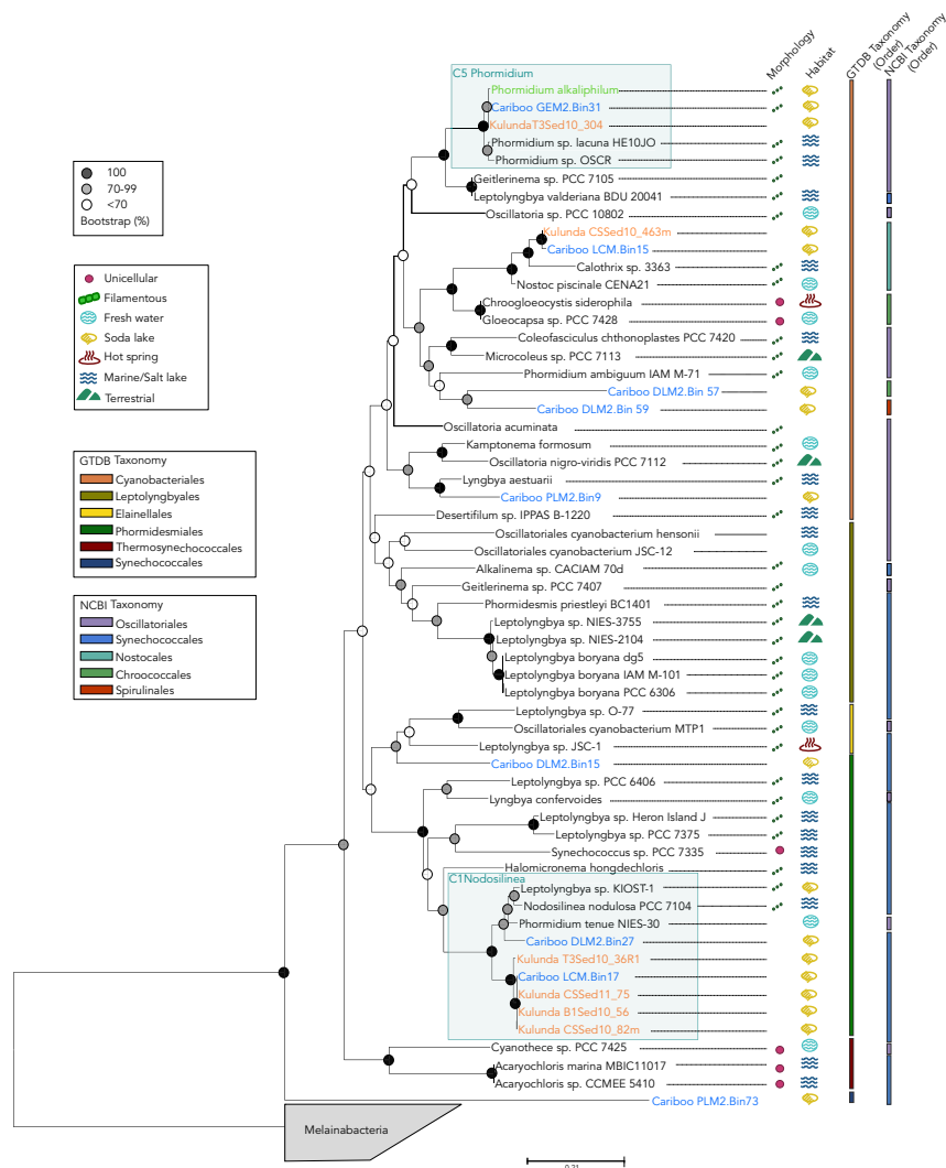
Figure 3. Maximum likelihood phylogenetic tree based on rpoABC amino acid sequences
