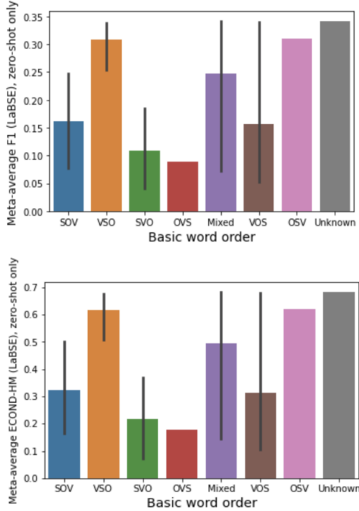
Figure 2: “Meta-average” performance of zero-shot languages with different word orders on F1-score and negative ECOND-HM (LaBSE).
