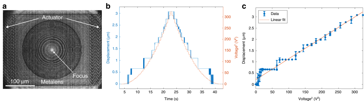
Fig. 2 Measured electrostatic actuation behavior of the MEMS platform. a Overlaid IR image showing both the device and focal planes of a singlet metalens on the MEMS-actuated platform. b Actuated focal displacement and applied voltage over time. The general trend of the actuated displacement follows the square of the applied voltage. c Average actuated displacement as a function of applied voltage squared during both loading and unloading, showing a linear dependence. No hysteresis behavior is observed with voltage loading and unloading, verifying the reversibility of the actuation process
