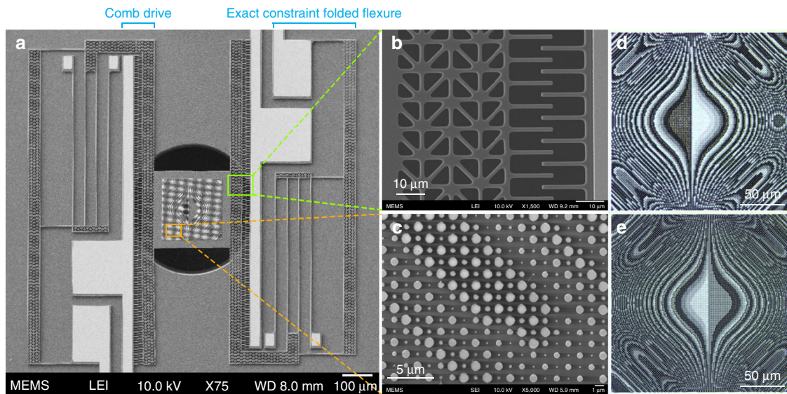
Fig. 1 SEM and optical images of a MEMS-actuated Alvarez metalens. a SEM image of a MEMS-actuated platform carrying the movable metasurface in an Alvarez metalens, with b and c being the zoomed-in SEM images portraying the electrostatic comb drive and the metasurface nanoposts, respectively. d, e Optical images of the Alvarez metasurfaces with complementary cubic phase profiles that are overlaid on top of each other in the assembled Alvarez metalens and in summation impart a quadratic phase change on the incident light
