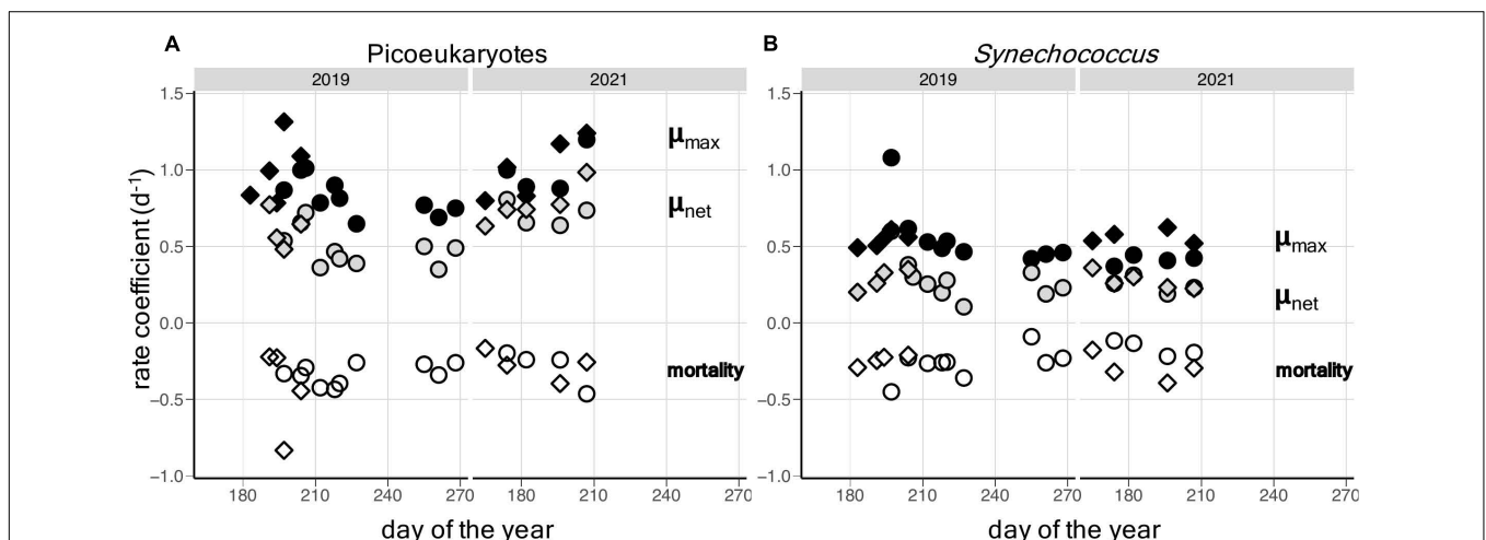
FIGURE 3 | Temporal patterns of net ( \mu_{net} ) and gross growth ( \mu_{max} ) rates and mortality due to grazing ( m ) in: (A) picoeukaryote; and (B) Synechococcus populations in Gulf of Maine coastal waters during the summers of 2019 and 2021. Values derived from saturation experiments are shown as circles and values from dilution experiments are shown as diamonds.
