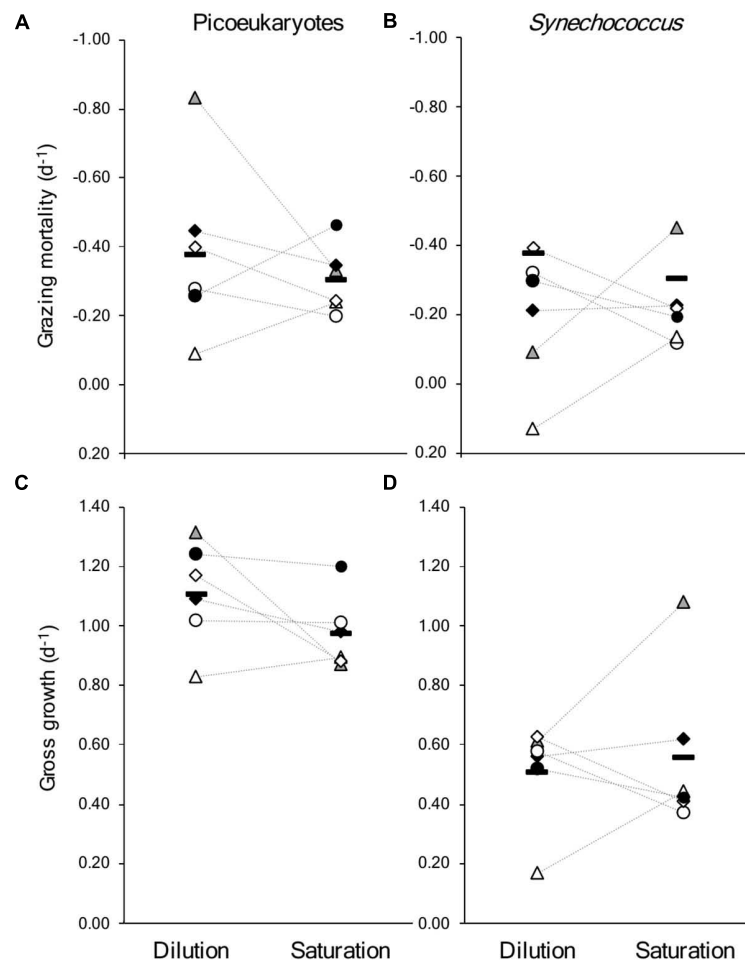
FIGURE 4 | Comparison of results from the six saturation and dilution experiments run in parallel in coastal waters of the Gulf of Maine in the summers of 2019 and 2021. Showing rates of mortality due to grazing for (A) picoeukaryotes, and (B) Synechococcus ; and gross growth rates for (C) picoeukaryote, and (D) Synechococcus . Paired symbols represent parallel experiments; gray triangle: day 197 (2019), black diamond: 204 (2019), open circle: 174 (2021), open triangle: 182 (2021), open diamond: 196 (2022), filled circle: 207 (2022); the horizontal bars are the mean of the six experiments, the dotted lines connect experiments run on the same day. The values and associated levels of uncertainty are included in Table 2 and Supplementary Tables 1, 2 . The dilution approach generated a positive slope for the relationship between apparent growth and level of dilution for Synechococcus on day 182 ( Supplementary Table 1 ).
