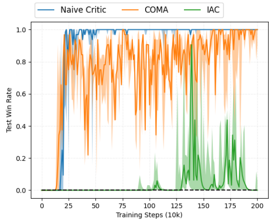
Figure 4: 2s_vs_1sc (Ablation 1)
