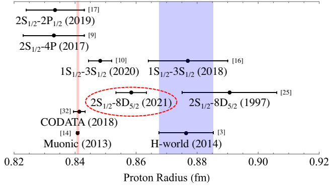
FIG. 4. A selection of recent determinations of the proton radius when combining laser spectroscopy with the 1S_{1/2} - 2S_{1/2} transition [9,10,16,19,40]. The result presented here is circled. The r_p denoted by H-world (2014) corresponds to the proton radius obtained in Ref. [3] using only hydrogen spectroscopy data (Adj. 8 Table XXIX). Also shown are the proton radius determinations from Lamb shift measurements in hydrogen [17] and muonic hydrogen [14], along with the most recent CODATA value [43].
