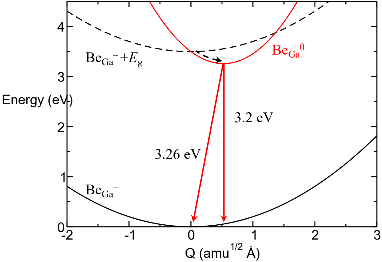
FIG. 7. (Color online) Configuration coordinate diagram for the shallow state of the \text{Be}_{\text{Ga}} acceptor. In the ground state, acceptor is negatively charged. The photogenerated hole is efficiently captured (dashed arrow) to the shallow state of the acceptor, with subsequent radiative transitions calculated to have the PL maximum at 3.2 eV and the ZPL at 3.26 eV.
