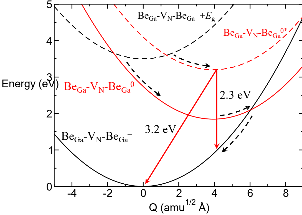
FIG. 13. (Color online) Configuration coordinate diagram for the \text{Be}_{\text{Ga}}\text{-V}_{\text{N}}\text{-Be}_{\text{Ga}} complex. In semi-insulating or n -type samples, the defect is negatively charged. The photogenerated hole can be captured (dashed arrows) either to the ground state of the hole, i.e., the neutral state \text{Be}_{\text{Ga}}\text{V}_{\text{N}}\text{-Be}_{\text{Ga}}^0 , or to the excited state \text{Be}_{\text{Ga}}\text{-V}_{\text{N}}\text{-Be}_{\text{Ga}}^{0*} . The transition via the ground 0/- level of the \text{Be}_{\text{Ga}}\text{-V}_{\text{N}}\text{-Be}_{\text{Ga}} complex is predicted to be nonradiative. The transition where the electron recombines with the hole in the excited state is radiative with the PL maximum of 2.3 eV and ZPL of 3.2 eV.
