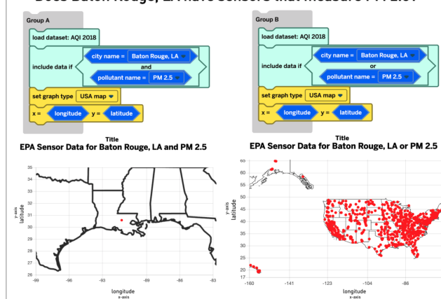
Figure 4: The Critiquing Code discourse routine (top) and an example Critiquing Code task in Data Studio (bottom)
