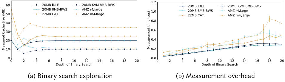
Fig. 4. Selection of the binary search depth.
