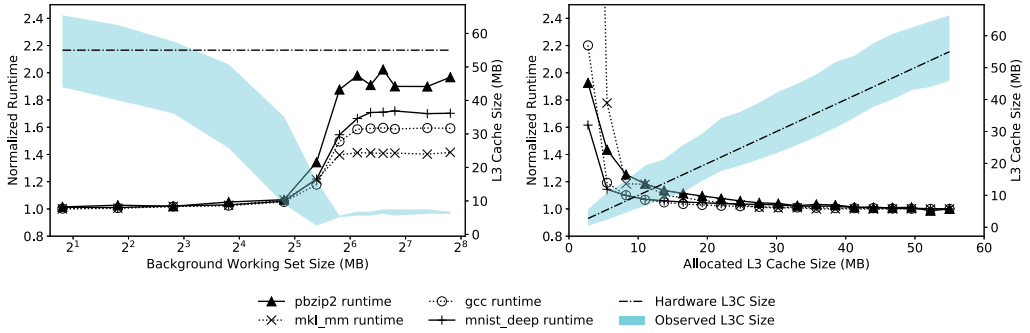
Fig. 1. Application performance with unmanaged cache contention (left) and with cache partitioning (right). The blue belts show the L3 cache range measured by CacheInspector .
