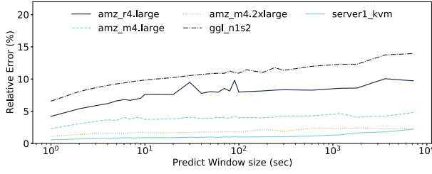
Fig. 13. L3 cache capacity prediction error.
