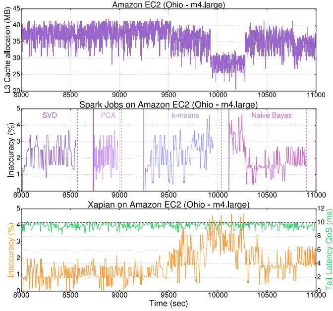
Fig. 14. Switch between precise and approximate execution for several Spark jobs (top) and the Xapian [45] search engine (bottom) under varying L3 cache allocations. When the allocated cache is below the requirement for nominal performance, the system sacrifices some output quality for reduced resources and improved execution time.
