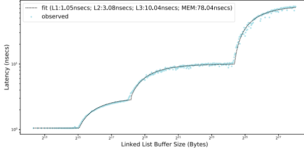
Fig. 3. Cache latency measurement and curve fit using the latency model derived from Equations (1) and (2).
