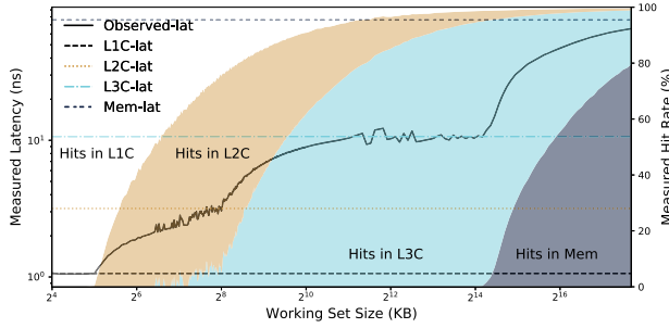
Fig. 6. Determining cache latency and hit ratio. The observed latency rises dramatically when the working set size grows beyond the cache boundary. The stacked hit ratio shows the percentage of the cache level in which memory accesses are ultimately served.
