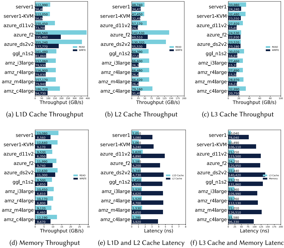
Fig. 8. Cache and memory performance in a controlled environment and three public cloud providers.
