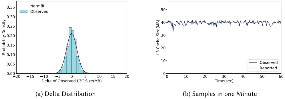
Fig. 12. Continuous L3 cache sampling with an m4.large instance in the Amazon Ohio Region.
