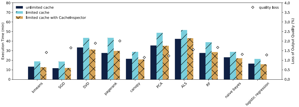
Fig. 15. Impact of reverse engineering the effective cache resources in a public cloud with CacheInspector .
