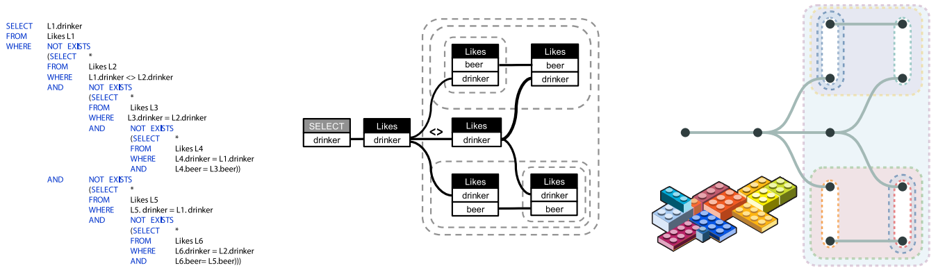
Fig. 2: Visualizing an SQL query (adapted from QueryVis, Fig. 1 [48]). Left: The SQL query for “find drinkers that like a unique set of beers.” Middle: The same query shown using QueryVis. Each table used is represented by a rectangle, subdivided vertically to show the title (black background) and relevant attributes (white background). The SELECT statement is similarly displayed, just with a gray background for the title. Curves show relationships between attributes (e.g., joins) and may be labeled with comparison operators (e.g., <> ). NOT EXISTS statements are shown as dashed lines surrounding hierarchically-nested groups for subqueries. Layers are arranged left-to-right to show depth from the SELECT statement, and the contained nodes are aligned to a vertical line. Right: An abstract representation of the QueryVis network, simplified by omitting any layout-irrelevant information (e.g., title nodes). The layout is optimized for readability using our method, with circles for nodes/attributes and nested convex hulls for groups. We illustrate which building blocks are used in the layout formulation (their arrangement is arbitrary).
