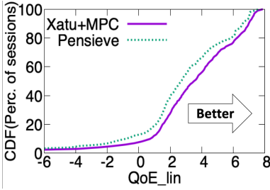
Fig. 10. QoE lin of Xatu+MPC and Pensieve from the testbed emulation. Note that many features of Xatu are disabled for fair comparison.
