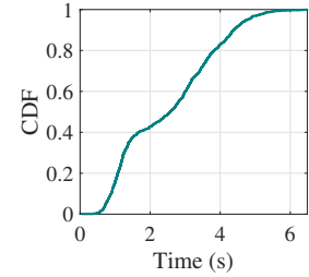
(b) CDF of total computation time.
