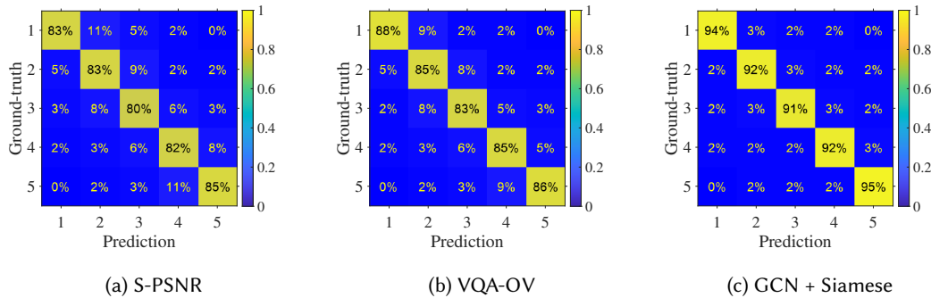
Figure 11. Advantage of GCN-based model - confusion matrix.
