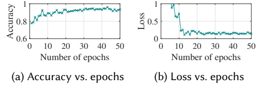
Figure 18. Convergence of MADA with respect to training epochs.
