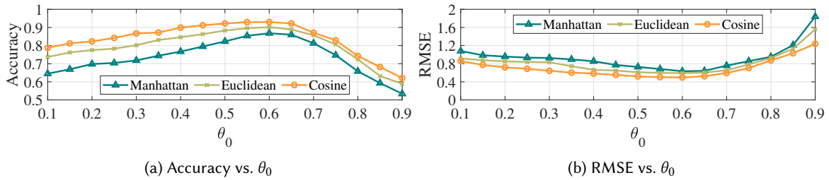
Figure 16. Impact of similarity metrics and \theta_0 's on prediction performances.
