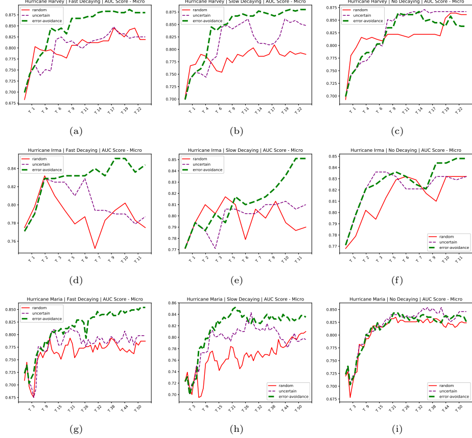
Figure 5: AUC score of mitigation algorithms for three hurricane datasets by various decay settings, showing superior performance of the proposed error-avoidance sampling in the case of memory decay errors.
