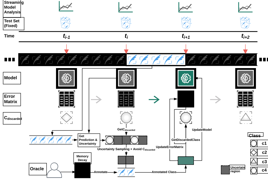
Figure 4: Summary of the proposed Error-Avoidance Sampling-based human error mitigation algorithm. At every interval, the streaming model predicts the potential class labels with uncertainty. The uncertain instances and instances of the discarded class label are filtered out, and the remaining are annotated by the oracle, which mimics the memory decay of human annotators. Based on the new annotations, the streaming model is updated, and the next class concept to discard is computed to avoid human errors in the annotation.
