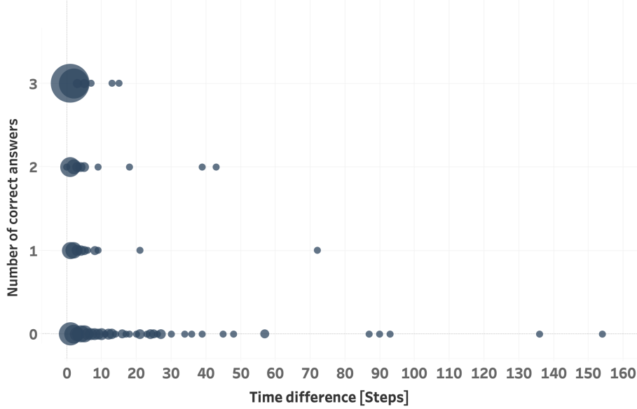
Figure 3: The temporal distribution of correct answers by human annotators shows a similar pattern as Figure 2 for memory decay behavior. The probability of incorrect answers (error) increases for annotating a given instance in the sequence with increased steps between instances of the same concept.
