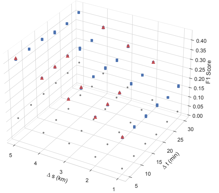
Fig. 3: We show the non-dominated set of solutions obtained through CROME (in red triangles). The learned CNN models are shown in blue squares. We also show the baseline models (in gray circles).
