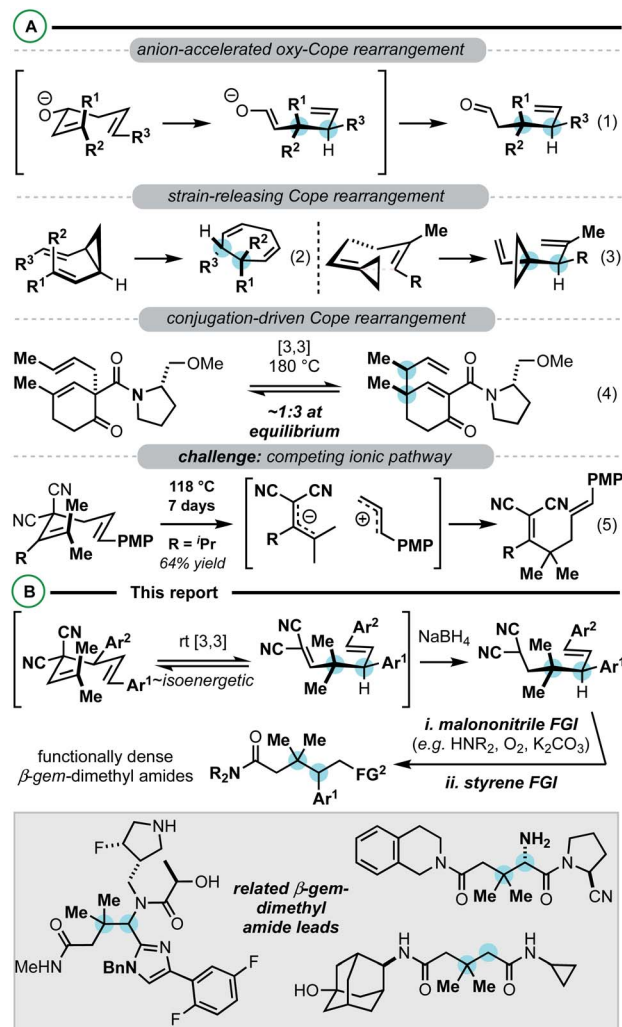
Scheme 1 (A) Cope rearrangements for constructing vicinal 4°/3°-centers (B) this report.
