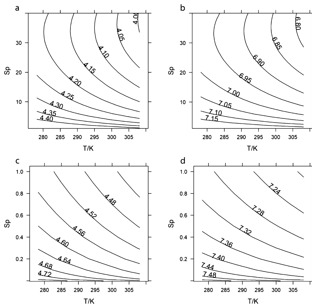
Figure 4. Dependence of pH on S_p and T , as calculated using the BCP algorithm of this study (eqs 1, 3, 4, and 5) and the minimum and maximum R values that can be reliably measured with a typical seagoing spectrophotometer. The upper panels (a,b) are for seawater, and the lower panels (c,d) are for freshwater. The left panels (a,c) are for the case of R = 0.05 , and the right panels (b,d) are for R = 20 .
