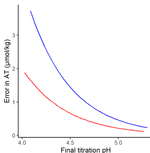
Figure 5. For single-step A_T methods, influence of the error in \log(K_2e_2) on uncertainty in derived A_T [using the equations of Liu et al. (2015) 2 ], expressed as a function of the final titration pH. A_T values were calculated over a range of R using \log(K_2e_2) values +0.01 and +0.02 units higher than the predicted value (eq 5). This figure illustrates the consequence of systematic pH errors [e.g., attributable to \log(K_2e_2) ] of 0.01 (red line) and 0.02 (blue line) on errors in derived A_T values.
