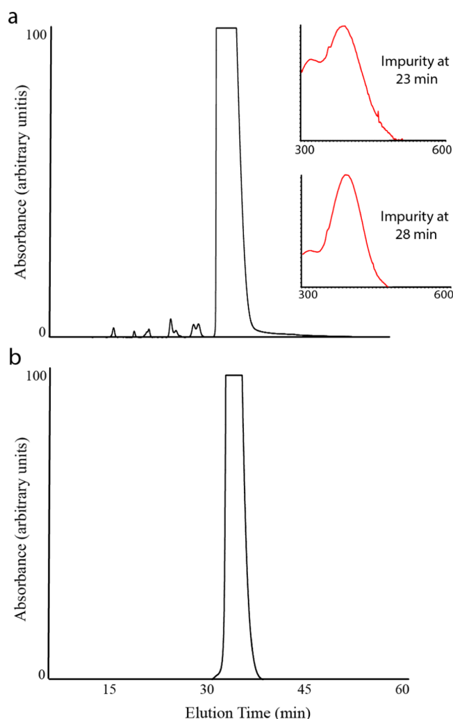
Figure 1. Chromatographs of off-the-shelf BCP (TCI batch WU III-FQ) before purification (a) and after purification (b) on the same scale using the Rediseq Gold C18Aq column. In panel a, the absorbance spectra of the impurities with an elution time of 23 and 28 min are expanded and shown in red. The combined integrated area of the impurities is approximately 1% of the pure BCP peak. Chromatographs of additional unpurified batches of BCP are provided in Figure S2.
