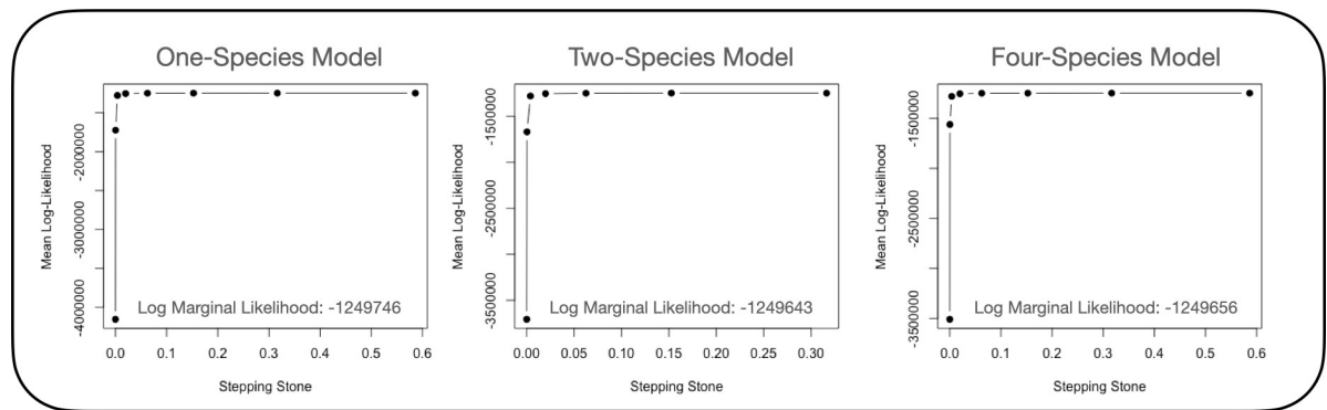
Fig 6. Species delimitation results for Poeciliopsis . Marginal likelihoods of the number of species in the ingroup sample calculated using the software BPP, and the R package bppr. Each point represents the mean log-likelihood calculated per stepping stone in BPP. The annotated likelihood in the lower right corner indicates the total marginal probability of the data. We used Bayes factor analysis to compare these marginal probabilities, concluding that the two-species model was more probable than the one-species model ( BF = 1.00 ) and the four-species model ( BF = 1.00 ).
