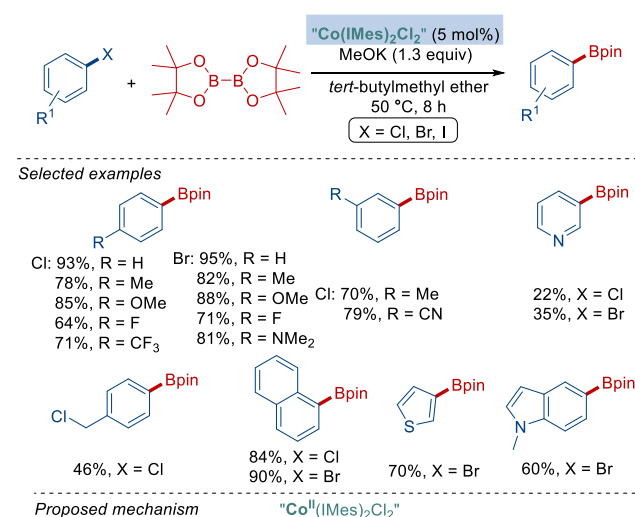
Scheme 17. Co-NHC Catalyzed Borylation of Aryl Chlorides and Bromides Reported by Geetharani.
