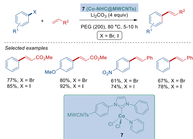
Scheme 16. Co-NHC Catalyzed Heck Reaction of Aryl Halides Reported by Hajipour.
