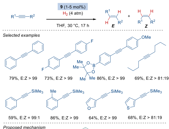
Scheme 21. Catalytic Semihydrogenation of Alkynes using Co-NHC CCC Precatalysts Reported by Fout.
