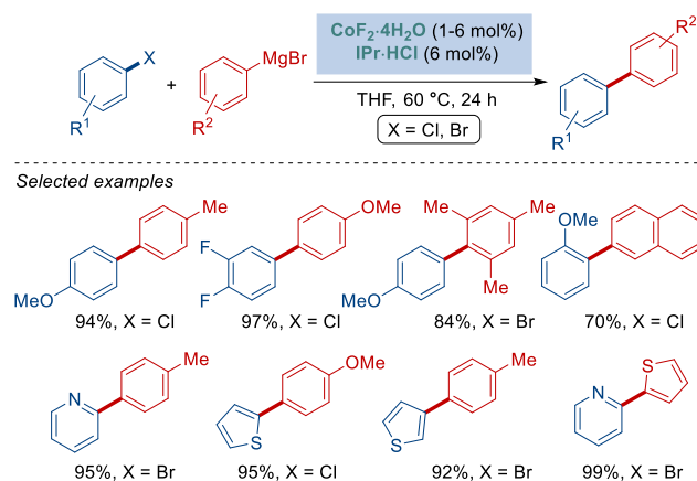
Scheme 7. Co-NHC Catalyzed Cross-Coupling of Aryl Halides with Aryl Grignard Reagents Reported by Duong.
