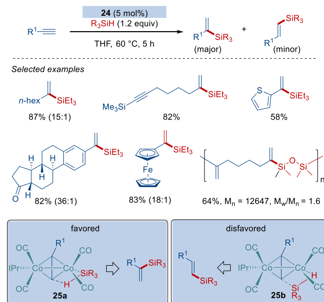
Scheme 36. Co-NHC Catalyzed Markovnikov Hydrosilylation of Alkynes Reported by Deng.
