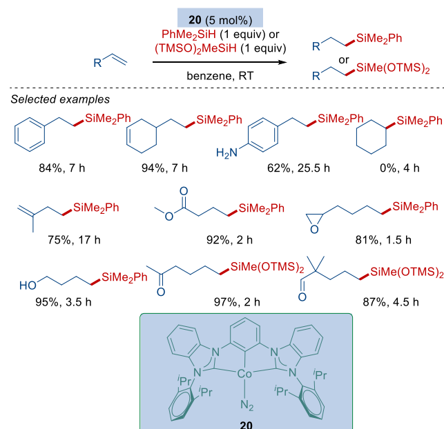
Scheme 33. Co–NHC Catalyzed Hydrosilylation of Alkenes Reported by Fout.
