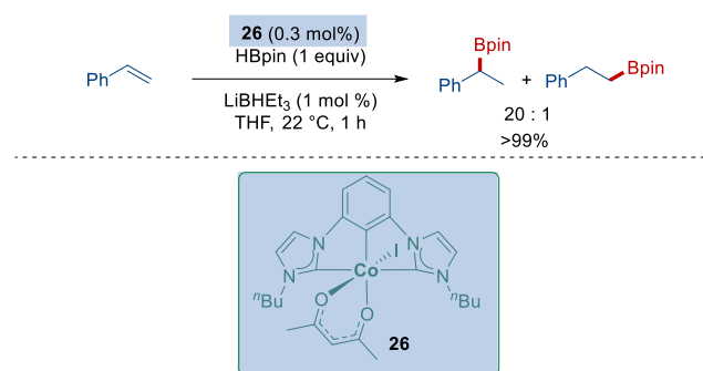
Scheme 38. Co-NHC Catalyzed Hydroboration of Alkenes and Nitriles Reported by Fout.
