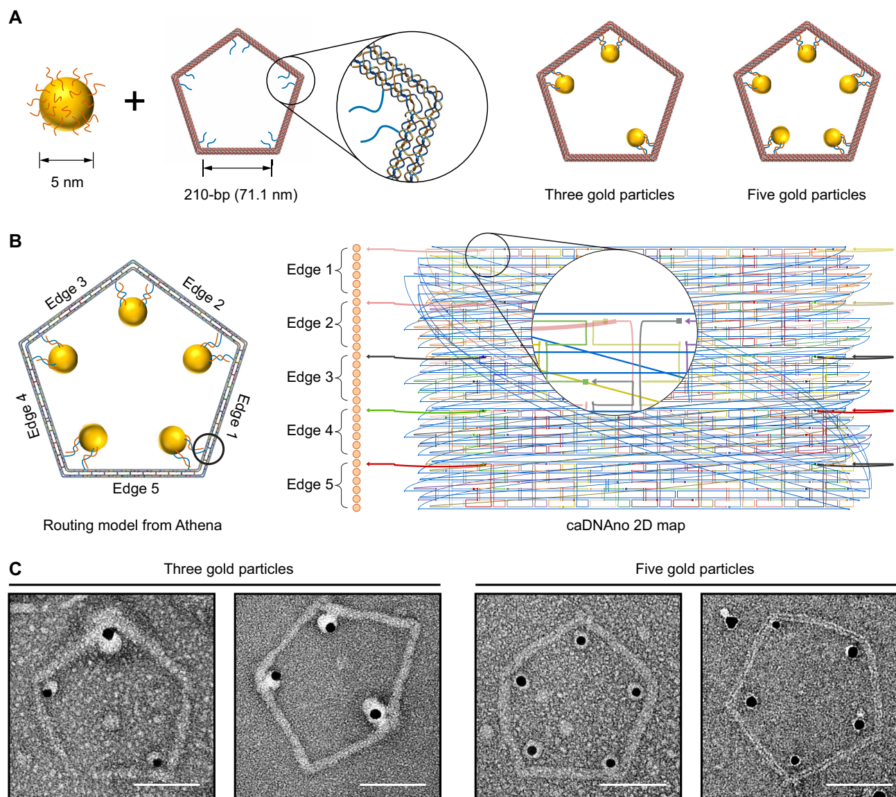
Figure 5. Organizing AuNPs on the 210-bp pentagonal DNA origami. (A) Diagrams showing the attachment of NPs at three or five corners. (B) Routing model and caDNA representation for pentagonal DNA origami with AuNPs. (C) TEM images with 2D pentagonal DNA origami of organized AuNPs. Scale bars, 50 nm.
