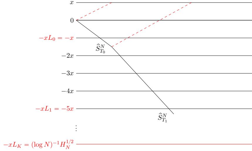
FIGURE 5.1. By the time the random walk \hat{S}^N exits the cylinder of radius (\log N)^{-1}H_N^{1/2} it has had about K independent opportunities to hit the level x , each with probability close to 1/2 .
