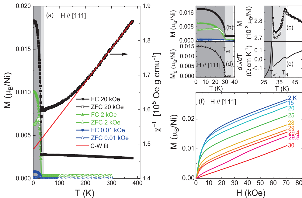
FIG. 2. (a) Temperature ( T ) dependence of the FC and ZFC magnetization ( M ) measured in 10-Oe (blue), 2-kOe (green), and 20-kOe (black) applied fields ( H ) along a [111] direction. FC and ZFC are shown as solid and open points, respectively. Plotted on the right axis are the 20-kOe data as inverse susceptibility ( \chi^{-1} = H/M ), along with a corresponding C-W fit (red line) between 200 and 380 K. As in panels (b)–(e), the dark and light gray regions correspond to the weak ferromagnetic and antiferromagnetic regions, respectively. (b)–(e) Low-temperature region T dependence of: (b) M in 10 Oe (blue), 2 kOe (green), and 20 kOe (black) [this is a close-up of the low- T behavior in (a)]; (c) M in 20 kOe; (d) M_0 as defined in (f); and (e) the T derivative of the apparent resistivity ( \rho ). The Néel temperature ( T_N ) and onset temperature for weak ferromagnetism ( T_{wf} ) are shown. (f) M(H) at various T between 30 and 2 K; these are magnetizing curves starting at H = 0 after ZFC to the shown T then warming above T_N before repeating. Linear extrapolation of the high- H ( >40 kOe) curves to H = 0 defines the M_0 plotted in (d).
