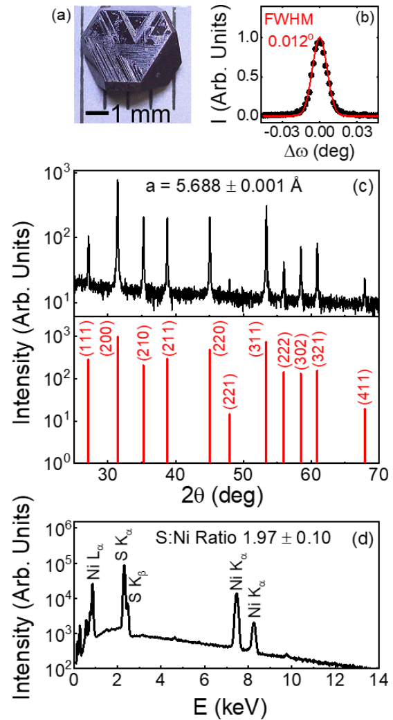
FIG. 1. (a) Photograph of a representative \text{NiS}_2 single crystal with a 1-mm scale bar. (b) 111 x-ray rocking curve of a typical \text{NiS}_2 single crystal, with the FWHM shown. (c) Wide-angle x-ray diffraction pattern from a representative ground \text{NiS}_2 crystal, with the expected pattern shown below. The deduced lattice parameter (from the sample height offset correction method) is shown, the error being from the associated fit. (d) Representative energy-dispersive x-ray spectrum from a \text{NiS}_2 single crystal, with the primary peaks labeled. The deduced S:Ni ratio of 1.97 \pm 0.10 (systematic-error dominated) is shown. The two most prominent unlabeled low-energy peaks are from (surface) C and O.
