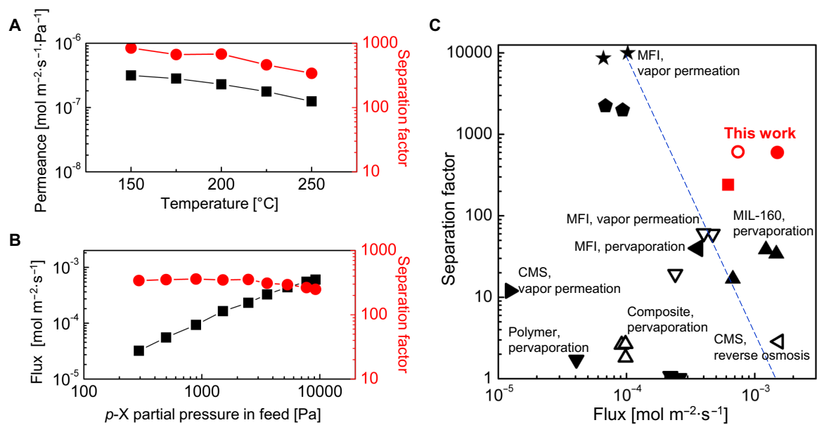
Fig. 6. Separation performance of zeolite MFI membranes for p / o -xylene binary mixture. (A) p -Xylene permeances and separation factors at various operation temperatures and (B) p -Xylene fluxes and separation factors at various p -xylene feed partial pressures (all mixtures with 1:1 p - and o -xylene) for a zeolite MFI membrane fabricated from a monolayer coating of novel (nanosheet-seeded) zeolite MFI nanosheets [membrane (D) in Table 1]. (C) Xylene isomer separation performance at 250°C for the zeolite MFI membranes reported here (○: membrane C, 7.7 kPa of p -xylene and 8.3 kPa of o -xylene in feed; ●: membrane C, 16 kPa of p -xylene and 1.7 kPa of o -xylene in feed; and ■: membrane D, 9.2 kPa of p -xylene and 9.9 kPa of o -xylene in feed) fabricated from the novel zeolite MFI nanosheets compared with other xylene isomer separation membranes from the literature [●: (30), ▽: (35), ★: (36), ►: (40), ◄: (41), ▲: (42), ◄: (43) ▼: (55), and △: (56)]. The dotted line shows the upper boundary for the performances of representative MFI membranes reported earlier.
