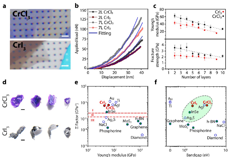
Figure 58. Mechanical properties of CrCl 3 and CrI 3 . (a) Optical microscopy images of 2L and few layers CrCl 3 and CrI 3 suspended over microwells (600 nm in diameter) on a SiO 2 /Si substrate. (b) Load–displacement curves and the corresponding fittings of 2L and 7L CrCl 3 and CrI 3 . (c) Volumetric Young's modulus and breaking strength of 2–10L CrCl 3 and CrI 3 , along with dashed lines that show the linear fits. (d) Demonstration of the good plasticity of bulk CrCl 3 and CrI 3 crystals via folding them into rings. (e) Deformability factor versus Young's modulus, where I, II, and III correspond to plastic-flexible, potentially deformable and brittle-rigid regions, respectively. The experimental results of CrCl 3 and CrI 3 are shown as red-filled circles, and the other layered vdW materials are shown as green filled circles. (f) Deformability factor versus bandgap for the same materials as in (e), and the materials that may show exceptional plastic behavior are shown in the dashed line encircled green area. 659 All panels are adapted with permission from ref 659. Copyright 2021 American Chemical Society.
