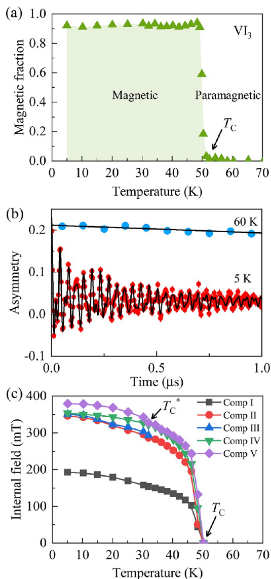
Figure 38. (a) Temperature dependence of the magnetic volume fraction for \text{VI}_3 , determined from weak transverse field \mu SR experiments. (b) Zero-field \mu SR spectra, recorded at T = 5 and 60 K. (c) The temperature dependence of the internal fields H_{\text{int}} for \text{VI}_3 . Original figure, no permissions needed.
