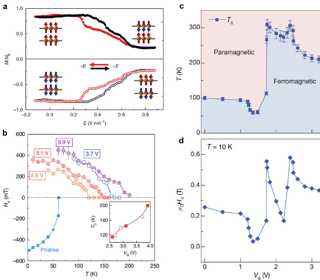
Figure 39. Voltage control of the magnetic properties of \text{CrI}_3 , CGT and FGT. (a) Top: Normalized magnetization measured by MCD as a function of the applied electric field (trace and retrace) at 4 K and fixed magnetic field (+0.44 T for top panel and −0.44 T for bottom panel), showing the electrical switching of the magnetic order in bilayer \text{CrI}_3 . The insets represent the corresponding magnetic states. 8 Adapted with permission from ref 8. Copyright 2018 Springer Nature. (b) Uniaxial magnetic anisotropy field ( H_u = H_s^\perp - H_s^\parallel ) of multilayer CGT as a function of temperature at different gate voltages and in the pristine case. Inset: The dependence of T_C on gate voltage. 86 Adapted with permission from ref 86. Copyright 2020 Springer Nature. (c) T_C of a trilayer FGT as a function of gate voltage. 12 (d) H_c of a trilayer FGT as a function of gate voltage at 10 K. 12 Panels (c) and (d) are adapted with permission from ref 12. Copyright 2018 Springer Nature.
