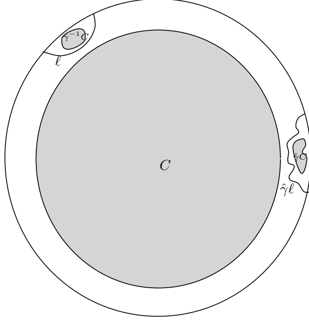
FIGURE 1. Depiction of the ingredients of the proof of Lemma 5.2. Here \hat{\gamma} := \rho(\gamma) .
