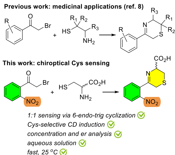
Figure 1. Development of a UV/CD sensing assay for D/L-cysteine mixtures.
