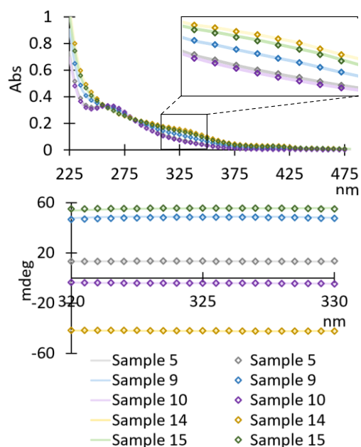
Figure 5. UV curves (top) and CD excerpts (bottom) of selected samples treated with 1 . See Table 1 and ESI for sensing results and details.
