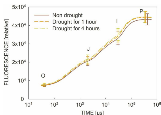
Fig. 1. Mean ChlF induction curves for three different drought stress levels (no drought, drought for 1 h, and drought for 4 h). The error bars are the standard deviations of O, J, I, and P points of the rice samples under the same drought stress level.
