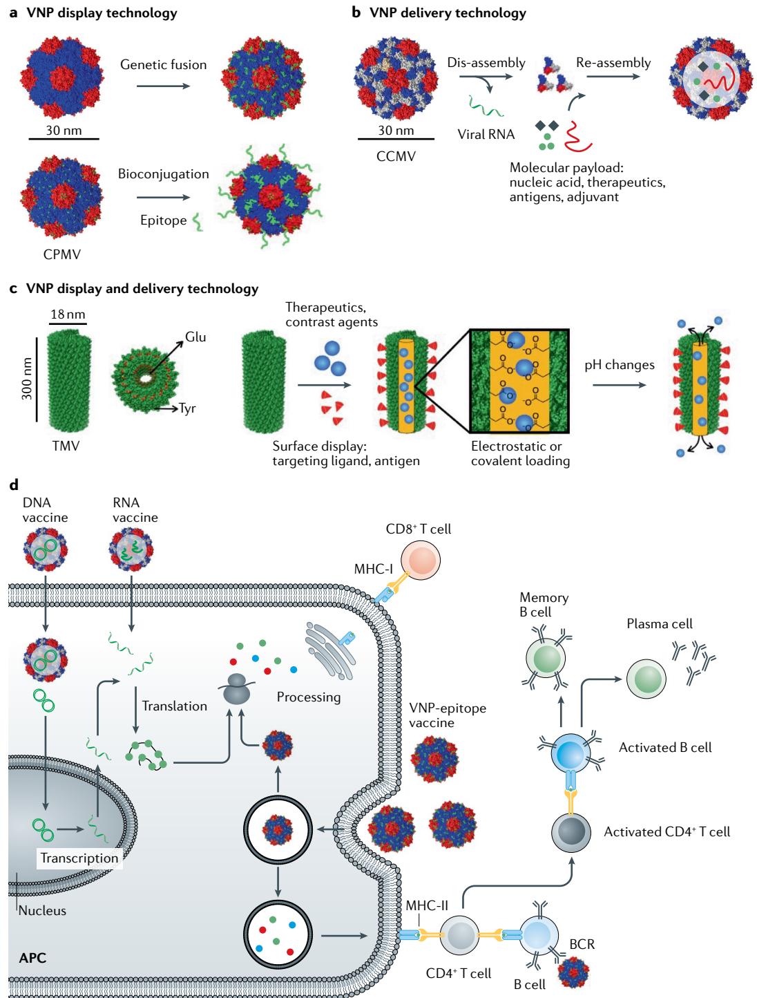
Fig. 2 | Structure and engineering design space of plant virus nanotechnologies and virus-like particle vaccines.
