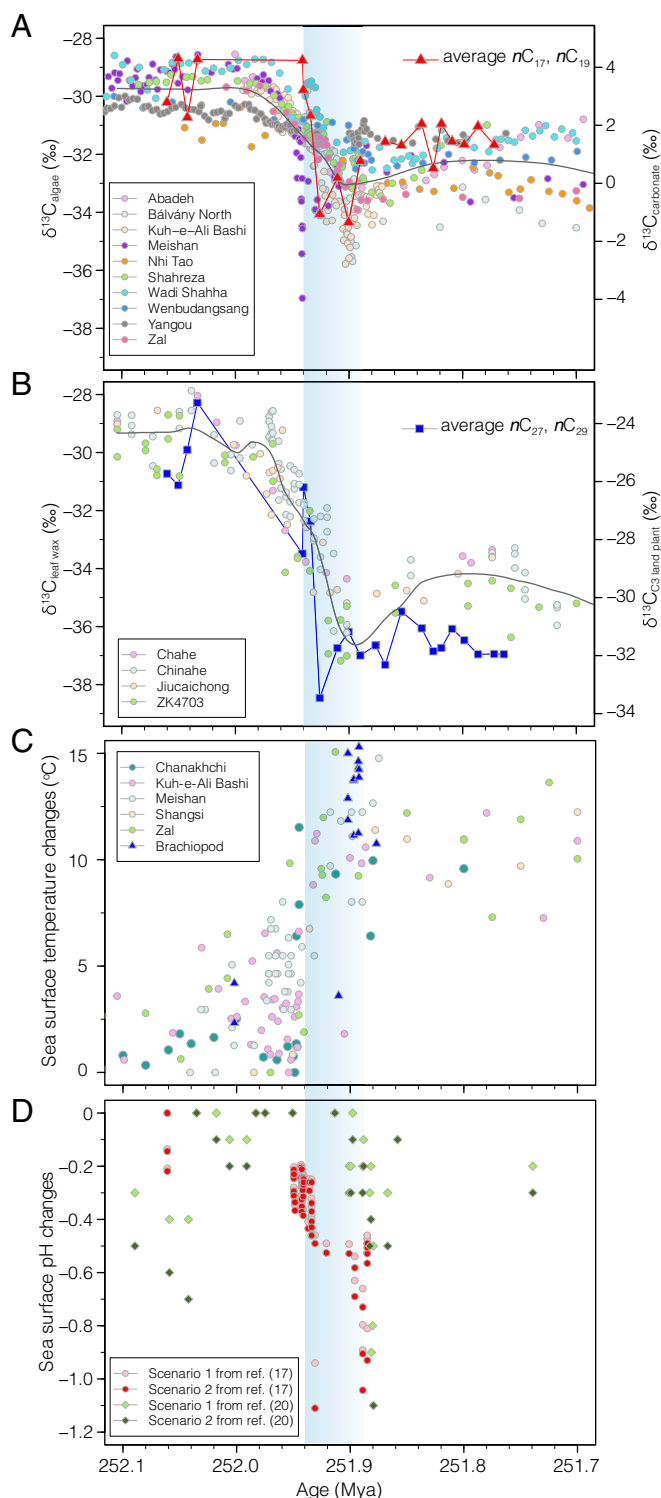
Fig. 4. Synthesized proxy records of carbon isotopes from marine carbonates and fossil \text{C}_3 land plants remains, sea surface temperature, and pH. (A) Comparison between \delta^{13}\text{C}_{\text{algae}} and global marine carbonate carbon isotopes from sites at Abadeh, Kuh-e-Ali Bashi, Shahreza, and Zal in Iran, Meishan, Wenbudangsang, and Yanggou in South China, at Bálvány North in Hungary, and at Nih Tao in Vietnam (24). (B) Comparison between \delta^{13}\text{C}_{\text{leaf wax}} and the \delta^{13}\text{C} of sedimentary leaf cuticles and wood of \text{C}_3 land plants from South China (24). (C) Reconstructed sea surface temperature data using conodont fossils (circles) (24) and brachiopods (triangles) (14). The conodont-based temperature data are from sites in the Paleo-Tethys, including Chanakhchi, Kuh-e Ali Bashi, Meishan, Shangsi, and Zal. (D) Relative changes in sea surface pH based on boron isotope proxy from ref. 17 and ref. 20. Pink and red circles are data
