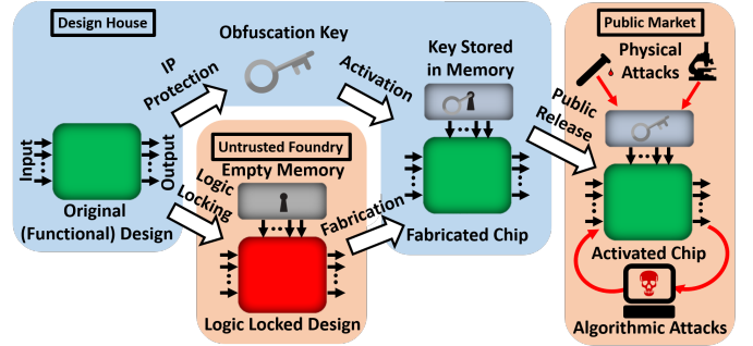
Fig. 1. Logic locking design flow. The logic-locked IC without the obfuscation key is secure from the untrusted foundry that fabricates it. The key is stored in non-volatile memory to activate the chip before release to the open market, where the key can be attacked through algorithmic and physical techniques.
