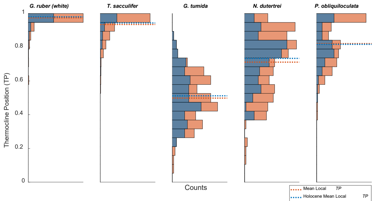
Figure 4: Local TP distribution for five tropical planktonic foraminiferal species for the full dataset and for Late Holocene dated data. TP = 1 corresponds to the surface, and TP = 0 to 1000 m. Numbers of data points for the full (“core top”) and Late Holocene (“Holocene”) datasets for each species are indicated. Dotted line represents mean of local TP estimates.
