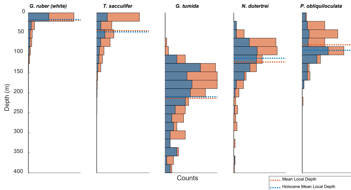
Figure 2: Local ACD distribution for five tropical planktonic foraminiferal species for the full core top data set and for Late Holocene dated (Chronozone 1-4) data. Dotted line represents mean of local ACD estimates.
