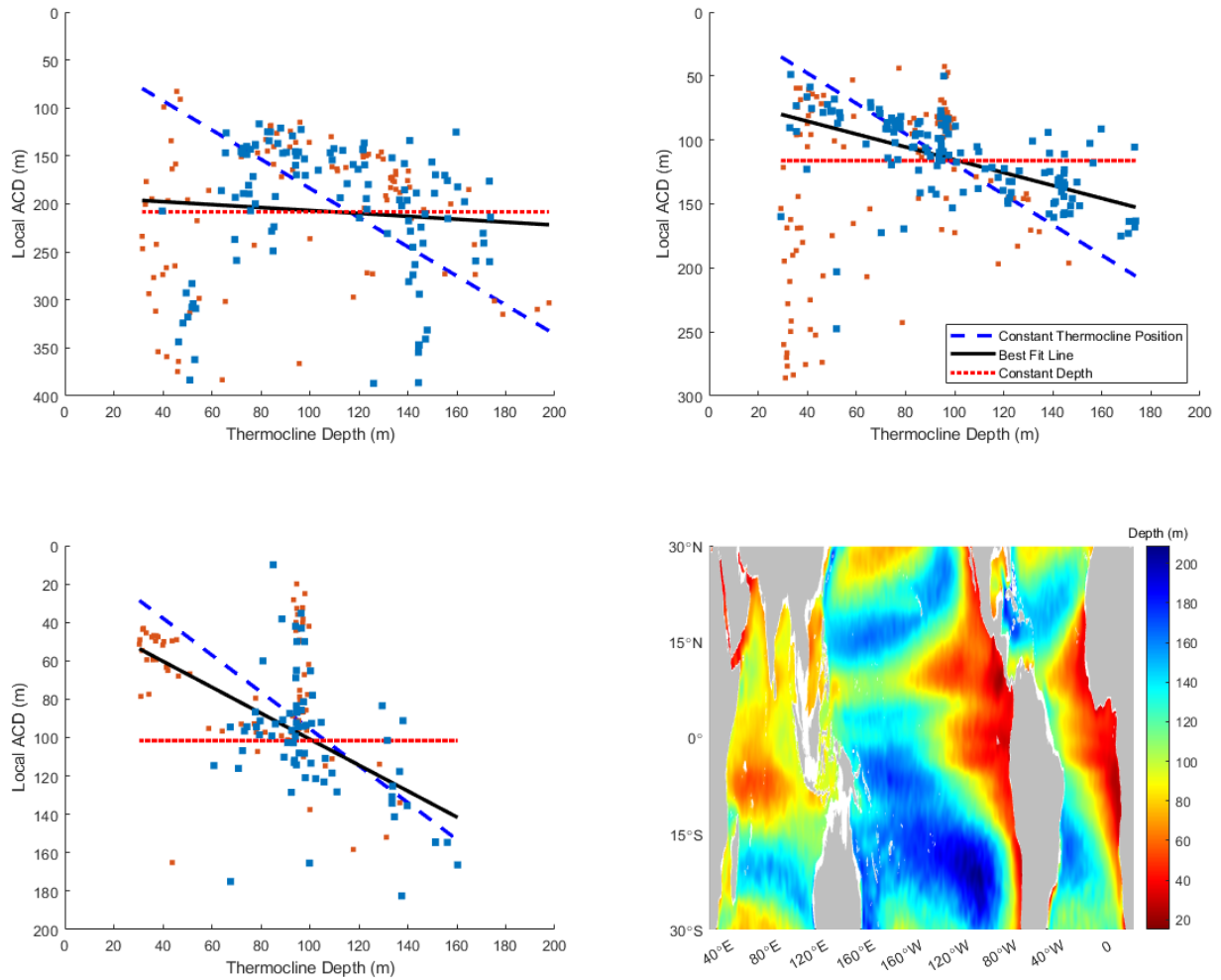
Figure 5: Local ACD calculated for G. tumida (a), N. dutertrei (b), and P. obliquiloculata (c) as a function of thermocline depth. Late Holocene data is shown in blue, and the full data set including core tops is shown in orange. Lines are best fit local ACD vs. thermocline depth (black), the expected local ACD for a constant average depth calcification (red), and the expected local ACD for a constant average thermocline position (TP) calcification (blue). d) Thermocline depth is defined as the depth where TP = 0.8 which approximates the thermocline depth.
